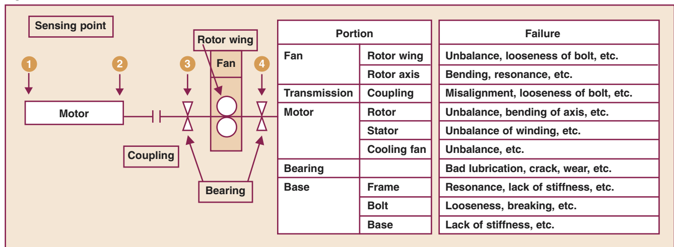
Figure 4 – Failure of air fan
