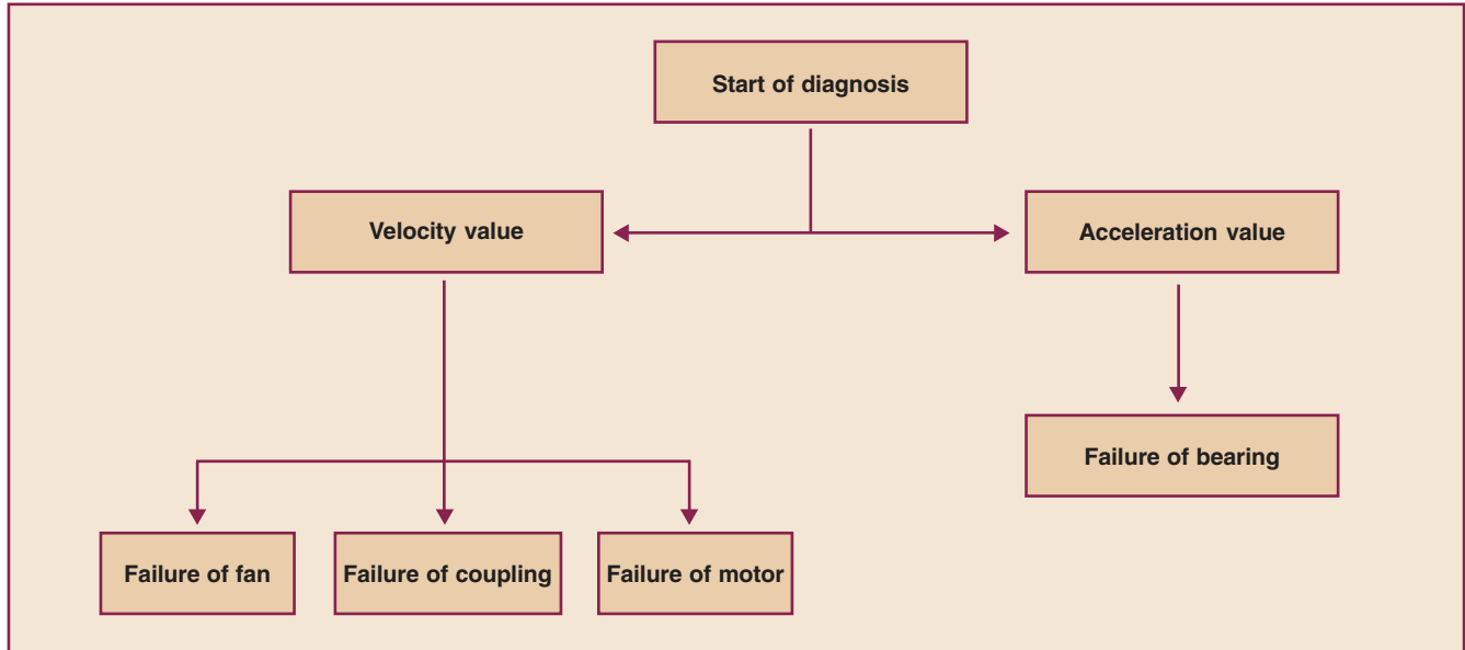
Figure 6 – Process of inference
