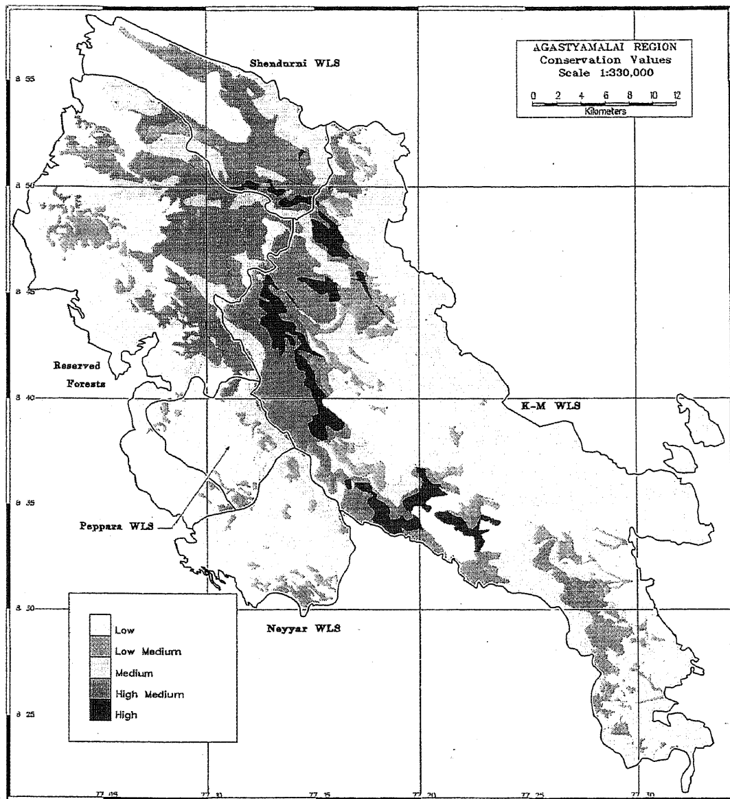
Figure 6. Map of conservation values in the Agastyamalai region of the Western Ghats.
