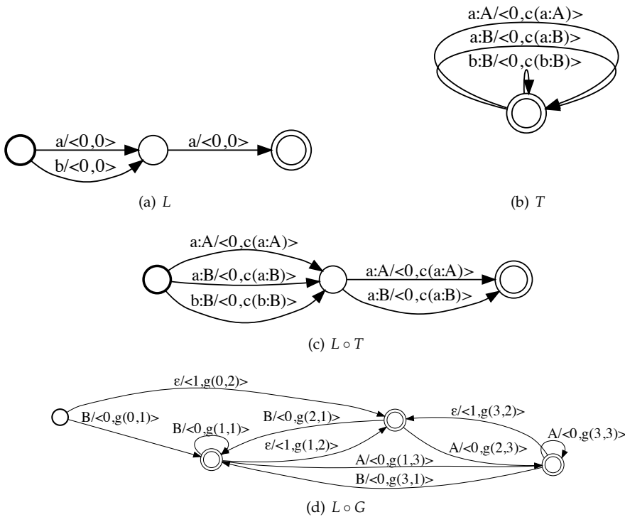
Figure 13 Input unweighted lattice L and tag mapper transducer T in \langle \mathcal{T}, \mathcal{T} \rangle semiring, where c(x:Y) is the cost of word x with tag Y . When composed, L \circ T yields a lattice of word:tag sequences. G is a tag language model, which encodes the smoothed transition probabilities of the HMM tagger. \epsilon represents backoff transitions; and g(x, y) gives the cost of transitioning from state x to state y in the model. Again, costs are in the \langle \mathcal{T}, \mathcal{T} \rangle semiring, so that backoff transitions have a cost of 1 in the first dimension.
