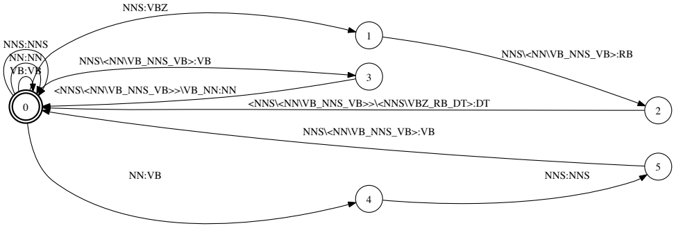
Figure 12 After conversion of the \langle T, C \rangle lattice back to the tropical, this mapper will convert the lattice to its final form.
