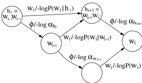
Figure 1 Deterministic finite-state representation of n-gram models with negative log probabilities (tropical semiring). The symbol \phi labels backoff transitions. Modified from Roark and Sproat (2007), Figure 6.1.
