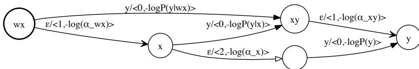
Figure 3 An example to illustrate the encoding of lexicographic language model semiring, where we set \Phi to 1. This is an instance of the general trigram LM depicted in Figure 1 with the sequence w_{i-2}w_{i-1}w_i = wxy . The scalar negative log probabilities are transformed from tropical semiring into tuples as explained in the text. The solid full, open, and unfilled full arrowheads correspond to the three cases—no backoff, bigram backoff, and unigram backoff, respectively.
