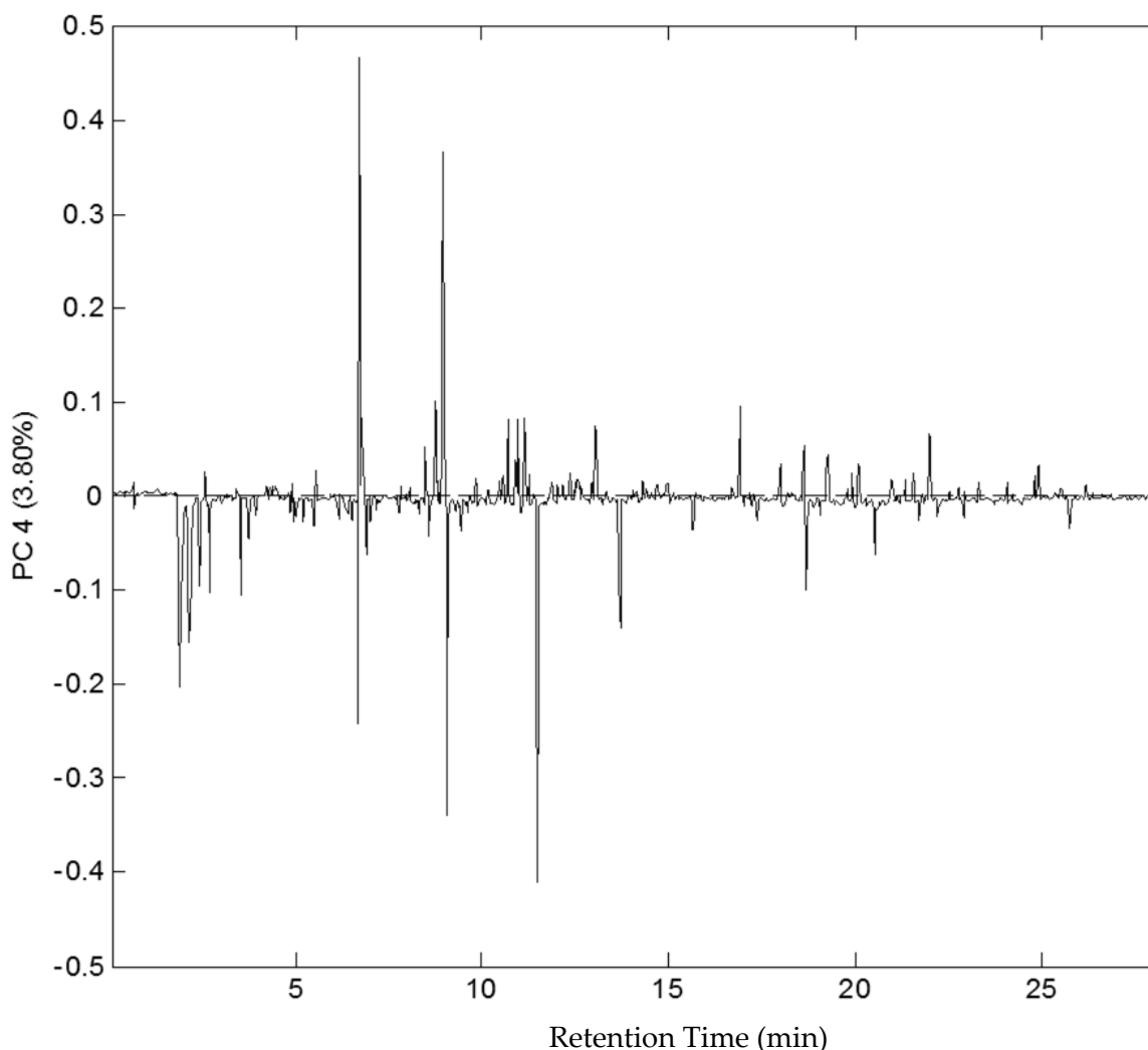
Figure 16. A loadings plot generated from a PCA model of silicone degradation pyrolysis data. Shown for example here is are the variables responsible for the 4 th principle component of the model.
