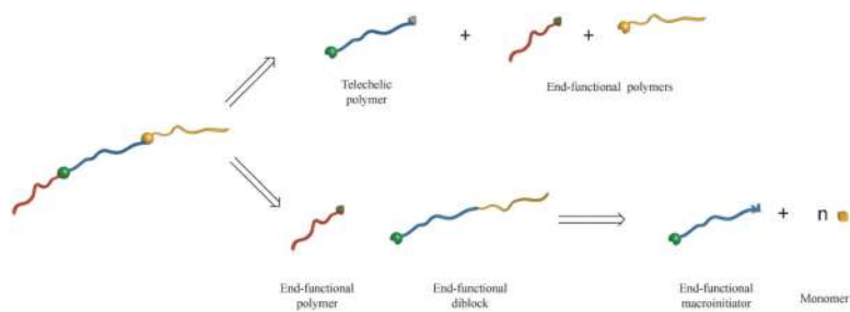
Figure 4. Retrosynthetic analysis for ABC triblock copolymers using REO chemistry by either a one-pot coupling of three unique mono- or hetero-bifunctional end-functionalized homopolymers (upper pathway) or by a step-wise growth and coupling of a homopolymer and diblock copolymer, each having a single complementary reactive chain end (lower pathway).
