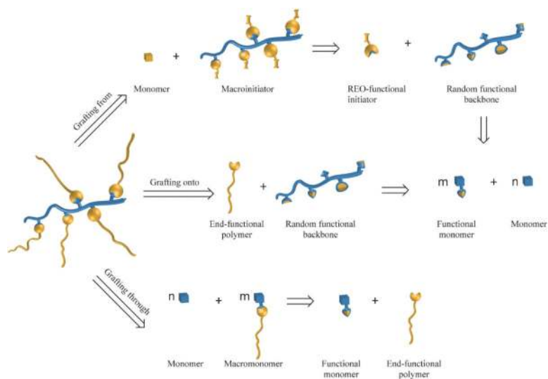
Figure 5. Retrosynthetic analysis for graft copolymers made using REO chemistry by the “grafting from” (upper), “grafting onto” (middle) or “grafting through” (lower) approaches.
