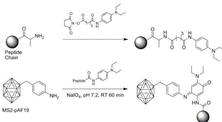
Scheme 71. Oxidative coupling of peptides to the exterior surface of MS2 viral capsids. 405
