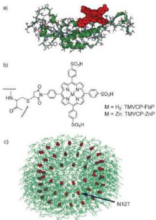
Scheme 69. Porphyrin-functionalized tobacco mosaic virus. 401 (Reproduced with permission from ref 403. Copyright 2007 Wiley-VCH).
