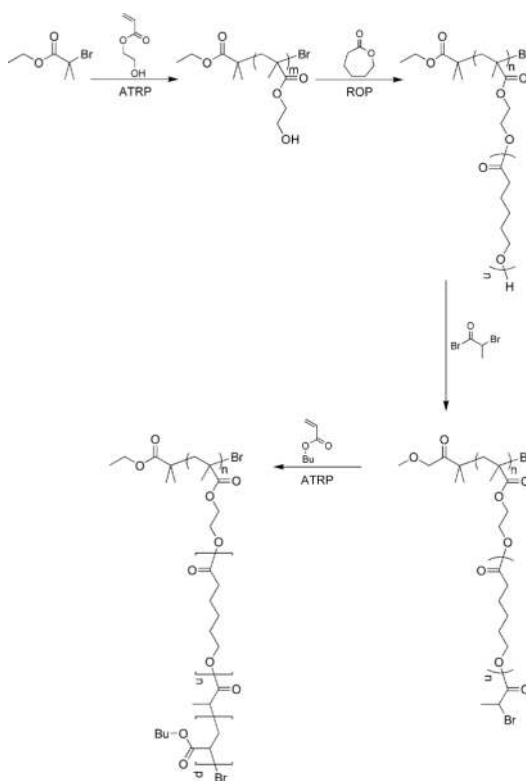
Scheme 12. Synthesis of a block graft copolymer with PCL- b -PBA side chains from a PHEMA backbone. 146
