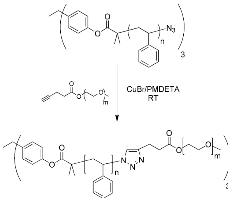
Scheme 34. Synthesis of PS- b -PEO three-arm star block copolymers by a combination of the “core first” and “coupling to” methods. 83
