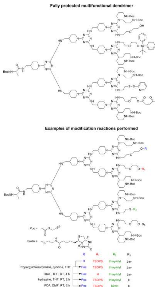
Scheme 45. Examples of multifunctional dendrimers from the group of Simanek. 212
