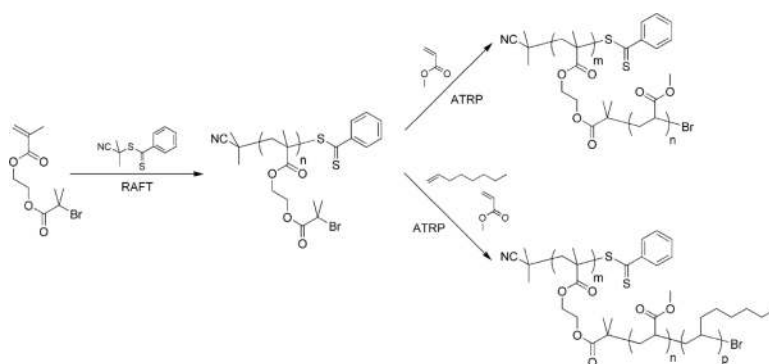
Scheme 13. Synthesis of a polymer brush with PMA and PMA-co-POct grafts using sequential RAFT and ATRP polymerizations. 147
