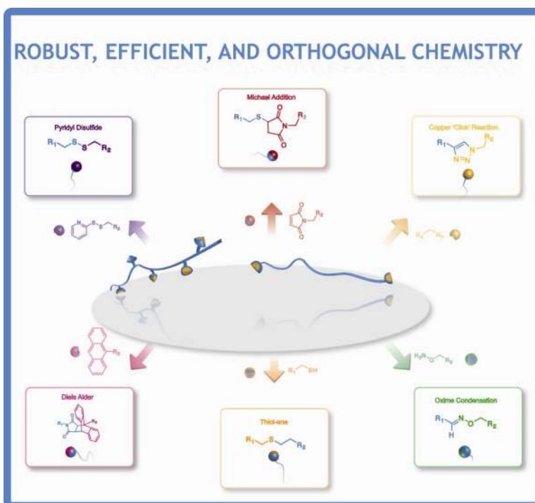
Figure 1. This article highlights examples employing “click” chemistry for the preparation and functionalization of complex polymer materials, three-dimensional substrates, two-dimensional surfaces, and biological systems. The types of chemical reactions include those that involve reactive functional groups, which undergo efficient, orthogonal couplings (REO chemistry), selectively and in high yield with limited by-products.
