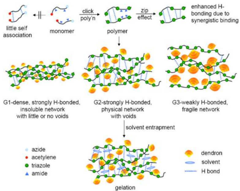
Figure 10. Gelation model for amphiphilic, dendronized polymers. 229 (Reproduced with permission from ref 231. Copyright 2008 Wiley-VCH).
