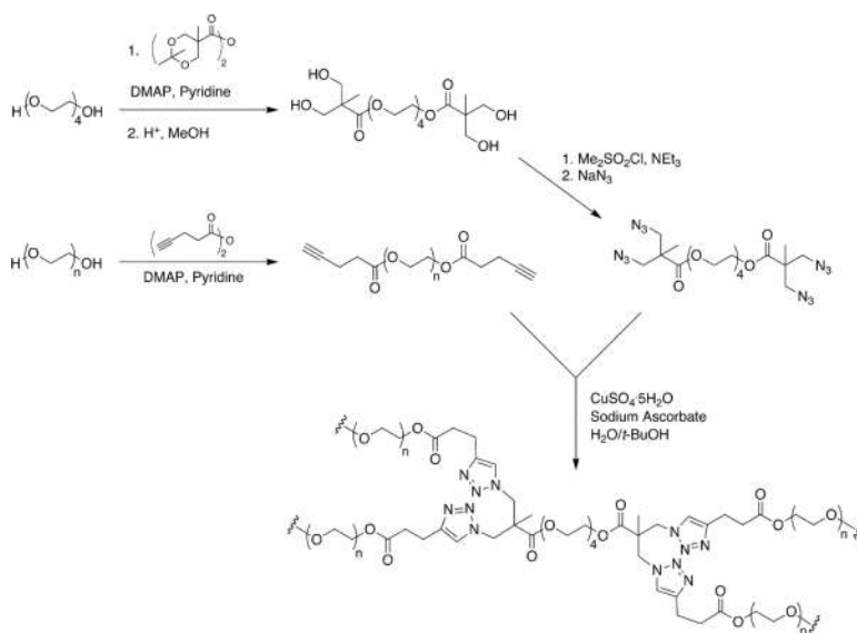
Scheme 49. The synthesis and formation of PEG-based hydrogels using CuAAC as the crosslinking reaction. 271
