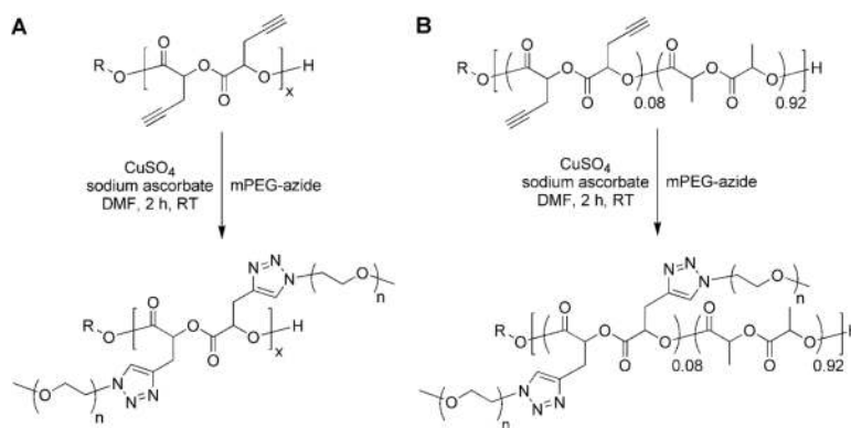
Scheme 24. Synthesis of A) PPGL- g -PEO homopolymer and B) (PPG- g -PEO)- co -PLA using CuAAC chemistry. 160
