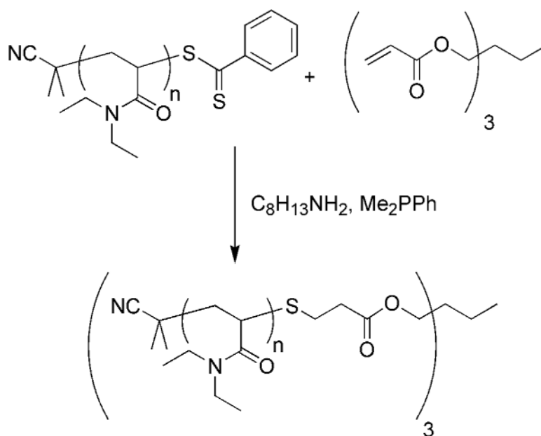
Scheme 30. Star polymer synthesis utilizing Michael addition of a dithioester-terminated linear polymer to a multifunctional diene core. 181
