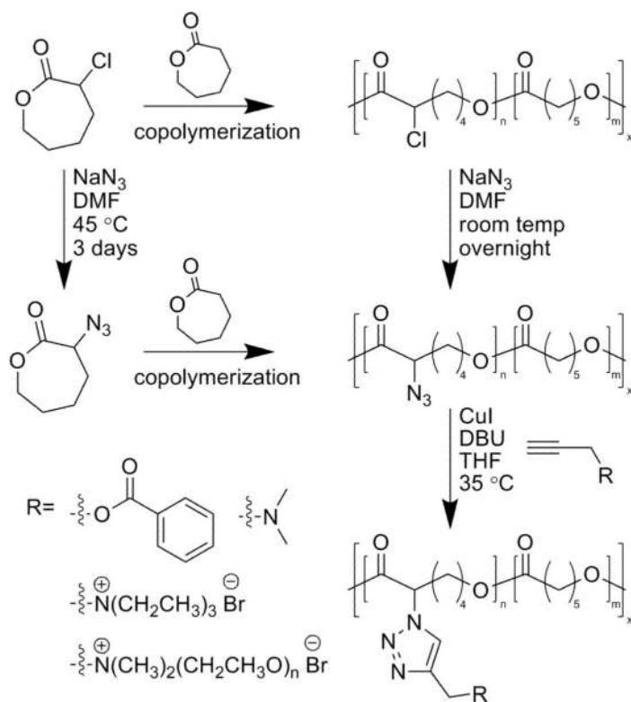
Scheme 8. “Click”able polyesters with a number of functional groups introduced. 112
