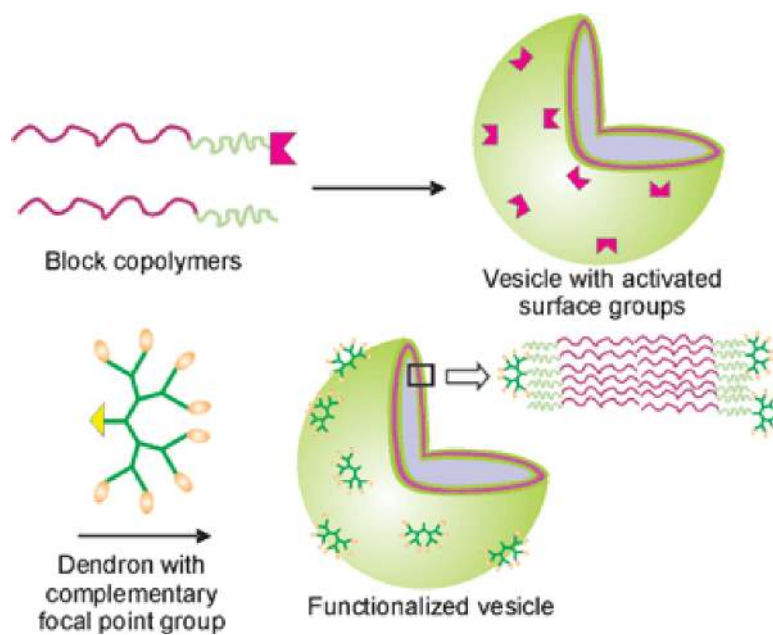
Figure 9. Conjugation of functional dendrons to a vesicle surface. 228 (Reproduced with permission from ref 230. Copyright 2007 The Royal Society of Chemistry).
