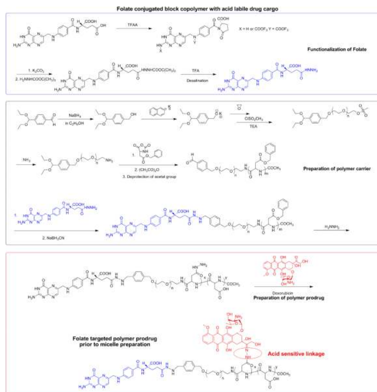
Scheme 56. Example of aldehyde-based strategies for preparation of folate receptor-targeted polymeric micelles with pH-sensitive drug cargos. 317
