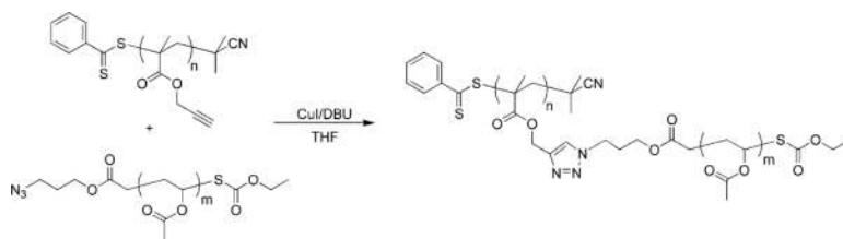
Scheme 20. copolymer prepared using RAFT, MADIX, and CuAAC cycloaddition. 156
