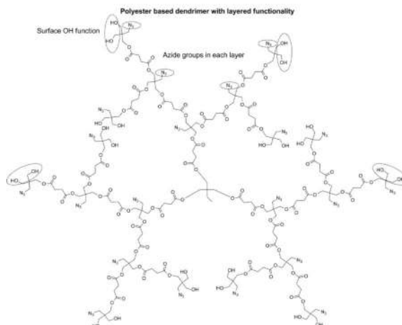
Scheme 43. Asymmetrically-functionalized polyester dendrimers (top), 208 and multifunctional polyester dendrimers (bottom) that allow for modification via orthogonal chemistry. 209
