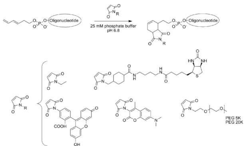
Scheme 75. Diels-Alder functionalization of oligonucleotides with PEG and various small molecules. 436
