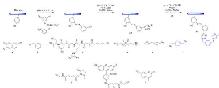
Scheme 67. Examples of 1,3-dipolar cycloaddition modifications of tobacco mosaic virus wires. 387
