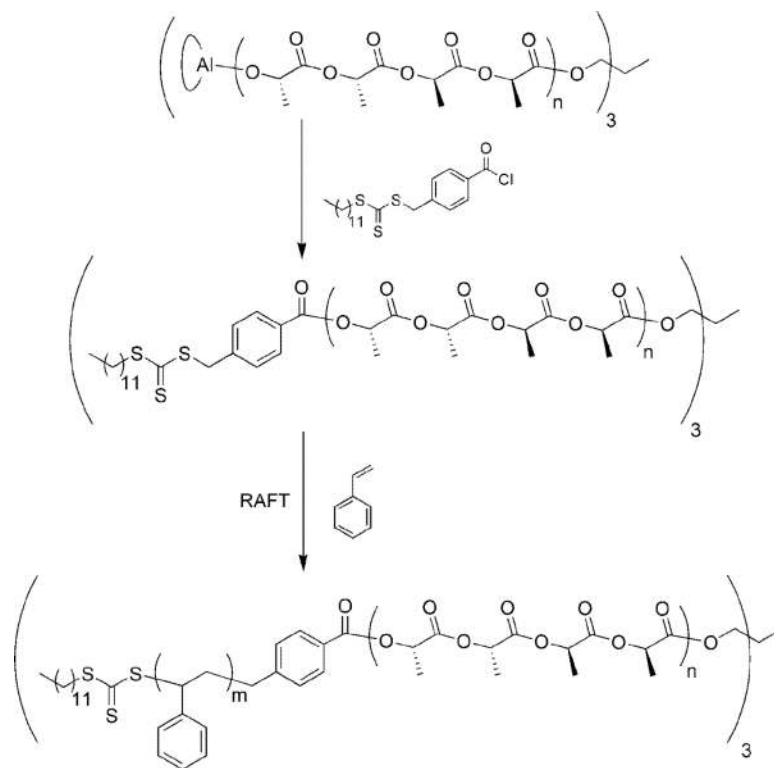
Scheme 33. Chain end functionalization with a RAFT chain-transfer agent and chain extension with styrene to yield star-shaped block copolymers. 182
