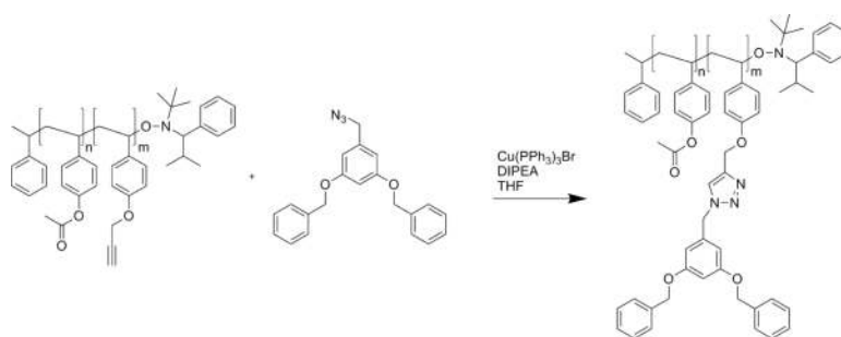
Scheme 47. Block copolymer containing dendronized blocks. 227
