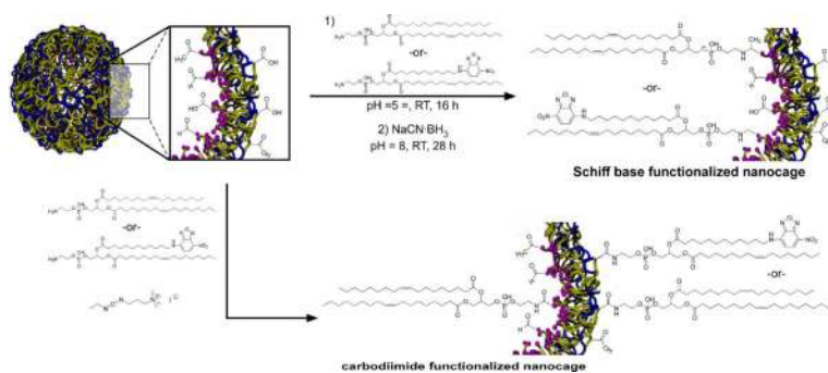
Scheme 58. Nanocage modification using amidation and reductive amination chemistries. 321
