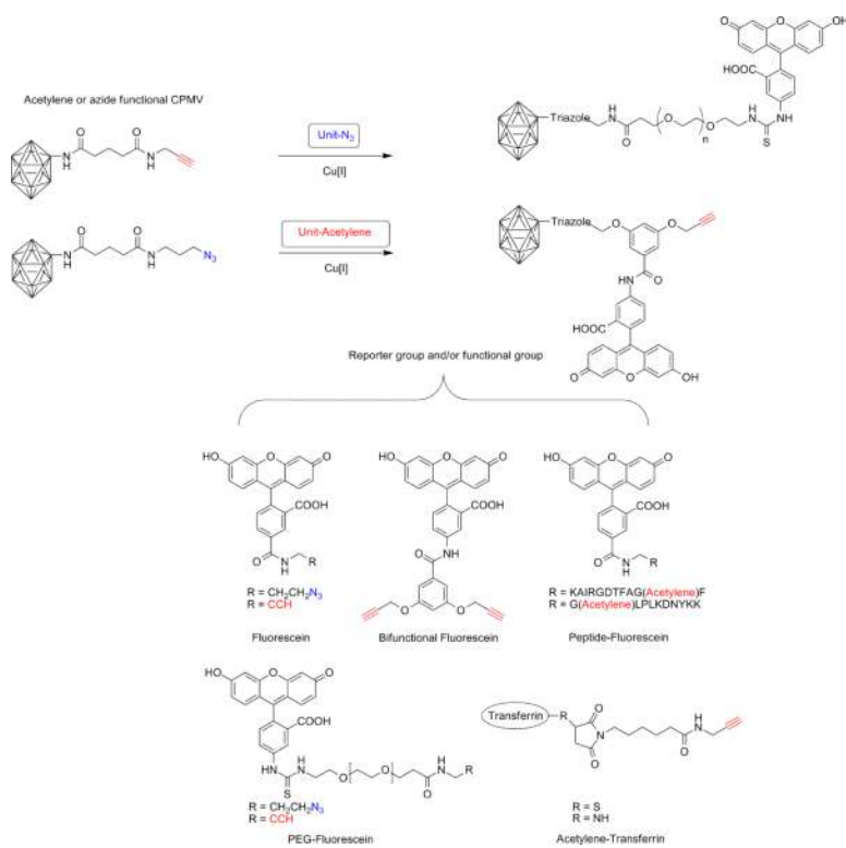
Scheme 66. Functional assemblies of CPMV particles and various functional units. 382
