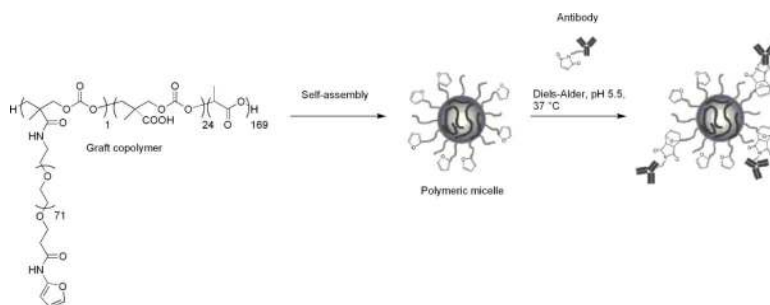
Scheme 60. Diels-Alder based functionalization of a polymeric nanoparticle with antibodies. 346 (Reproduced with permission from ref 348. Copyright 2007 Wiley-VCH).
