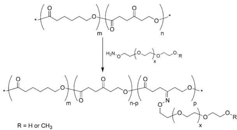
Scheme 25. Preparation of PCL-g-PEO using ketoxime ether formation. 131
