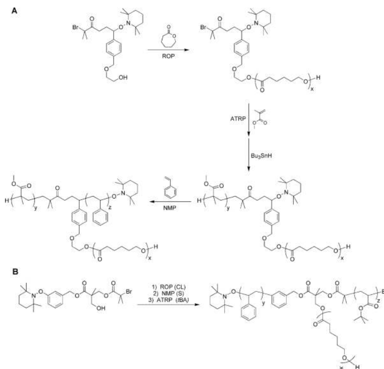
Scheme 37. Syntheses of ABC miktoarm stars employing ROP, NMP, ATRP and a “core-first” approach. 184,185
