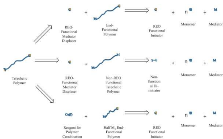
Figure 3. Retrosynthetic analysis for a homopolymer containing REO reactive groups at both chain ends. The upper method can produce heterobifunctional materials, while the bottom two methods can only successfully make homobifunctional polymers. In this example, a mediator represents some species that controls polymerization at the active end of a polymer chain ( e.g. halogen in ATRP, nitroxyl in NMRP, catalyst in ROP/ROMP, etc. ), and a 'non-functional' initiator is one that does not include a moiety capable of undergoing an REO transformation. In the case of ATRP, the halogen, which serves as the mediator, can be replaced by a nucleophile to give some useful end-group that can undergo an REO transformation ( e.g. organic azide).
