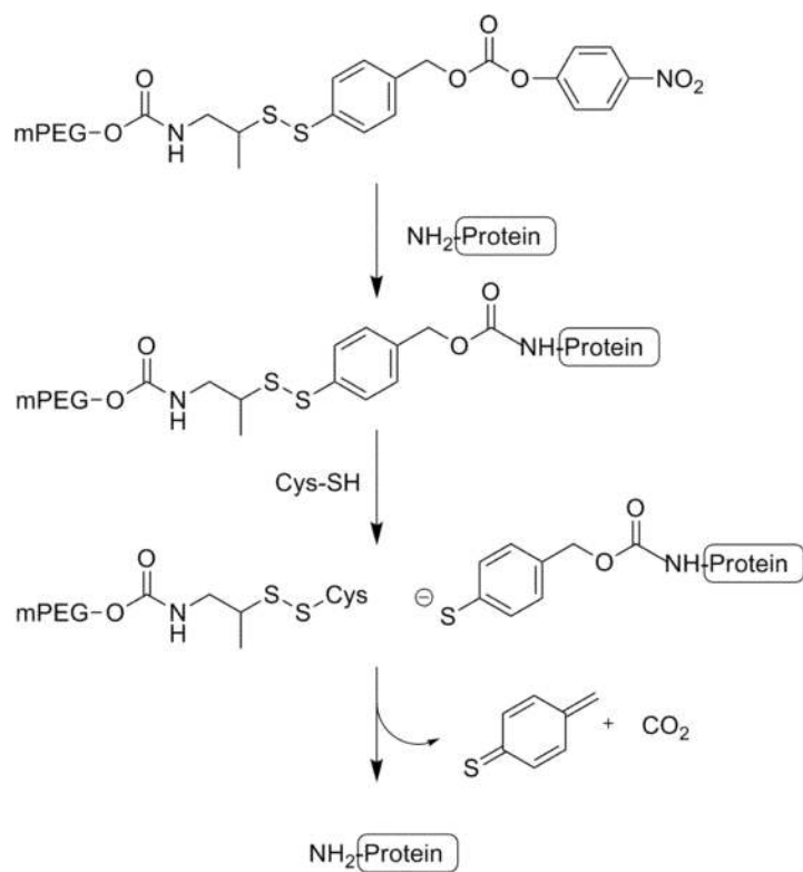
Scheme 74. PEGylation via the formation of thiol cleavable conjugates. 127
