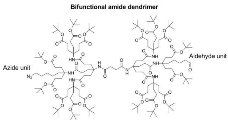
Scheme 44. Orthogonally-functionalized dendritic polyamides. 210
