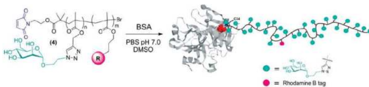
Scheme 72. Synthetic glycopolymers based on BSA. 42 (Reproduced with permission from ref 42. Copyright 2007 American Chemical Society).
