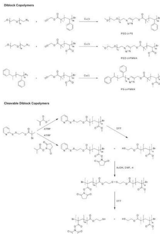
Scheme 3. Formation of diblock copolymers by CuAAC, and cleavable diblock copolymers using disulfide chemistry. 1,98
