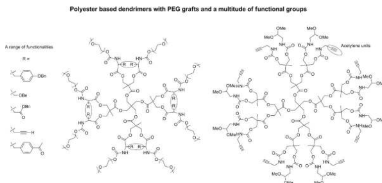
Scheme 42. Examples of multifunctional polyester dendrimer constructs for nanomedical applications. 206,207
