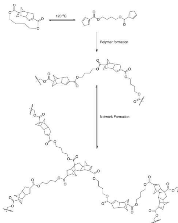
Scheme 52. Formation of self-reparable networks using reversible Diels-Alder reactions for crosslinking from a single component system. 285
