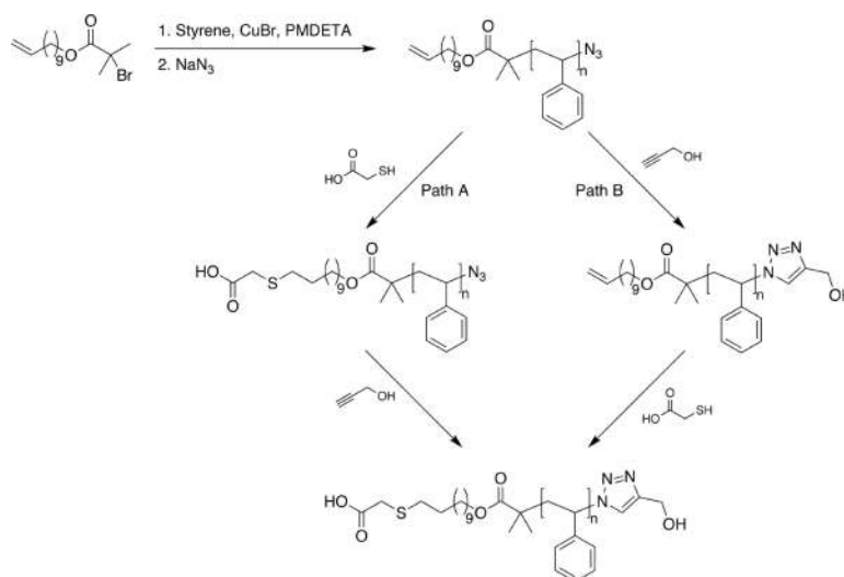
Scheme 5. Orthogonal functionalization of the \alpha - and \omega -chain ends of a polystyrene derivative using orthogonal thiolene and CuAAC chemistries. 46
