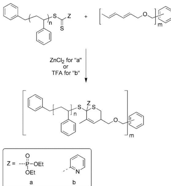
Scheme 29. Use of RAFT polymerization and subsequent hetero Diels-Alder reaction to construct two-, three-, and four-arm star topologies. 180
