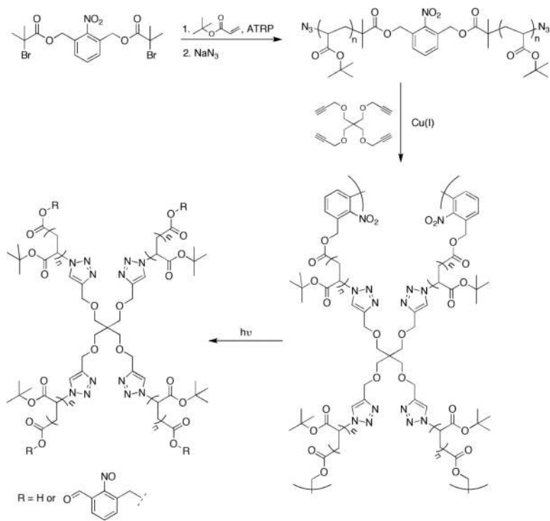
Scheme 50. Synthesis and degradation of photodegradable model networks made by ATRP and CuAAC. 84,85,275
