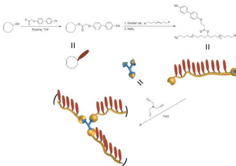
Scheme 51. Chemical strategy for construction of liquid crystalline networks crosslinked in a well-defined manner from metathesis-based telechelic polymers containing either 1 or 2 mesogens per repeat unit. 276
