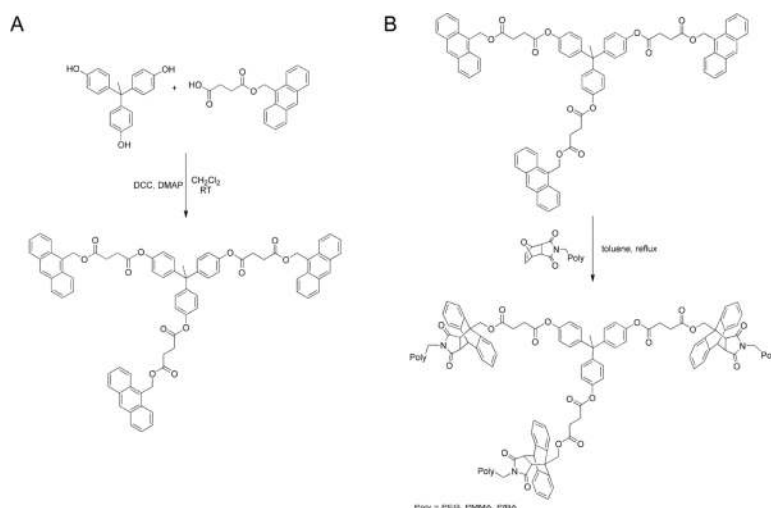
Scheme 28. Construction of three-arm star polymers using an anthracene-maleimide based Diels-Alder “click” reaction. 179
