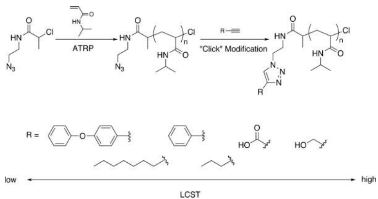
Scheme 1. Modification of the chain terminus of P(NIPAM) polymers derived from functional initiators and post-polymerization CuAAC chain end modification. This study revealed significant effects of only changing the end group on the LCST, which varied by over 10 °C. 37
