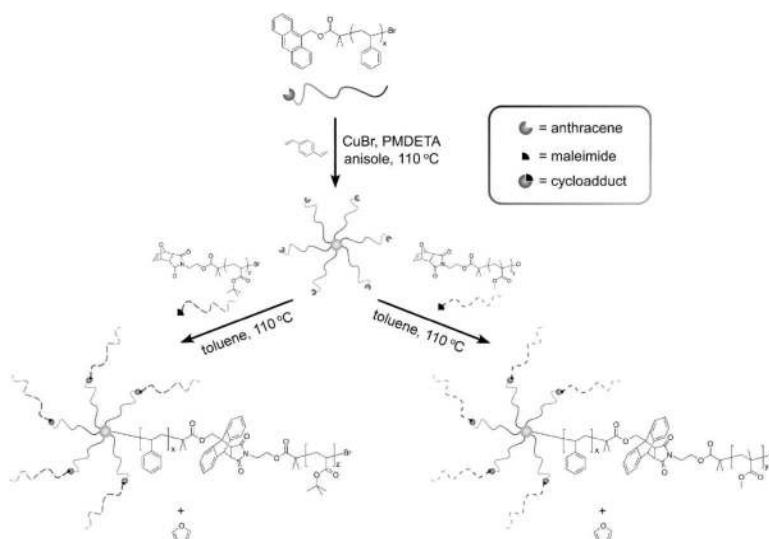
Scheme 35. Synthesis of multi-arm star block copolymers using the Diels-Alder “click” reaction between anthracene and maleimide derivatives. 35
