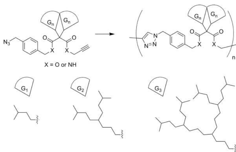
Scheme 48. Step polymerization of hydrocarbon based dendritic monomers through CuAAC chemistry. 229
