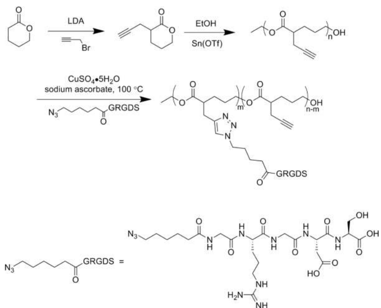
Scheme 9. Alkyne-functional polyesters allow for incorporation of biologically-active peptides. 113
