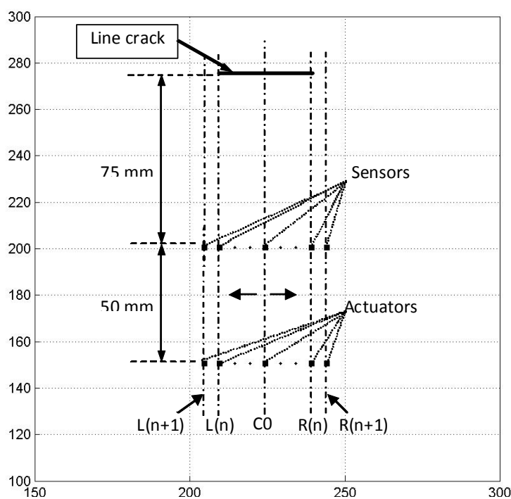
Figure 9. Quantification of damage extent (adopted from Figure 9 in [20]).
