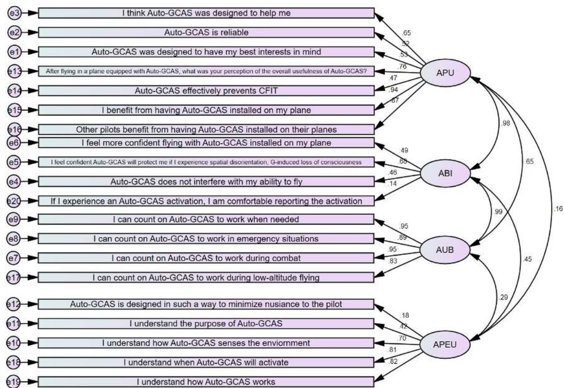
Figure 13. Measurement model CFA results of original proposed AGCAS-TAM with unacceptable fit and six standardized loading factors below minimum acceptable values.
