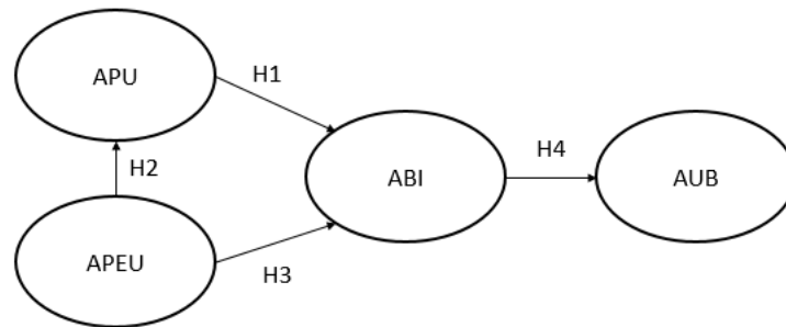
Figure 7. Graphic representation of the hypotheses between latent variables in the AGCAS-TAM.
