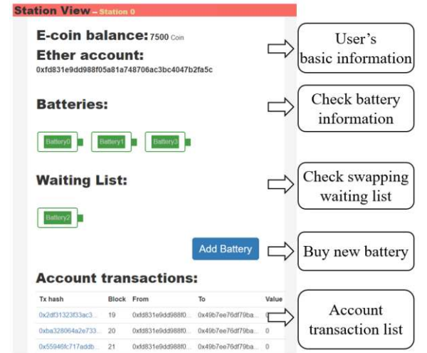
Figure 9. Index page of station operators
