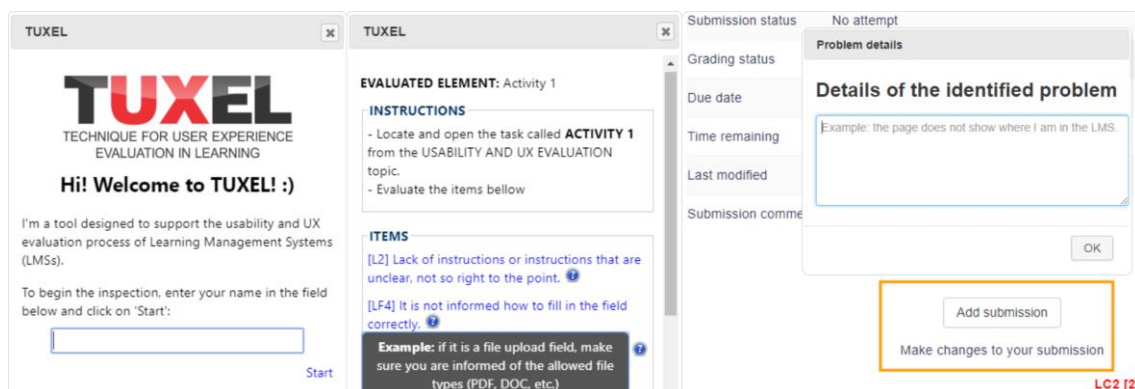
Figure 2. Screenshots of the interface of TUXEL 2.0 tool.
