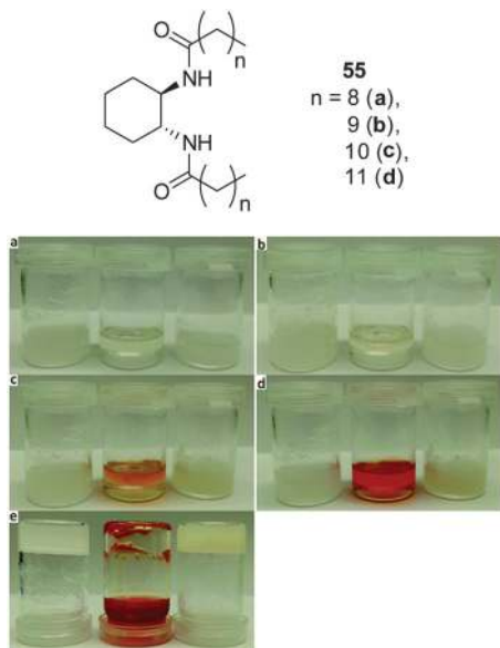
Fig. 35 Chemical structure of cyclohexyldiamide 55 and photographs of gels containing compound 55d (20 mg) and DMSO (1 mL), pyridine (1 mL) and TEA (1 mL). (b) The addition of DCP (0.1 mL) to the surface of gel samples. (c) 1 h 48 min after DCP addition. (d) 2 h 58 min after DCP addition. (e) 5 h 5 min after DCP addition showing gel breakdown and intense red colour. Figure adapted from ref. 101 with permission.
