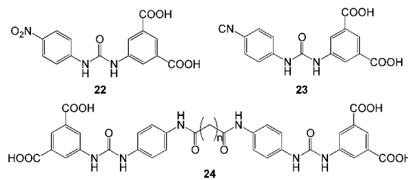
Fig. 15 Chemical structure of urea based gelators 22–24 developed by Hayes, Miravet, Escuder and co-workers for dye adsorption. 48,49
