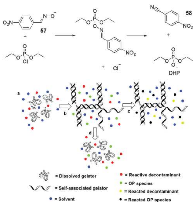
Fig. 37 4-Nitroaldehyde oxime 57 reactive nerve agent decontamination compound, the mechanism of its reaction with DCP to form 58 , and a schematic of how a gel incorporating reactive decontaminant can respond to the presence of nerve agents and act to remediate against them. Figure adapted from ref. 104 with permission.
