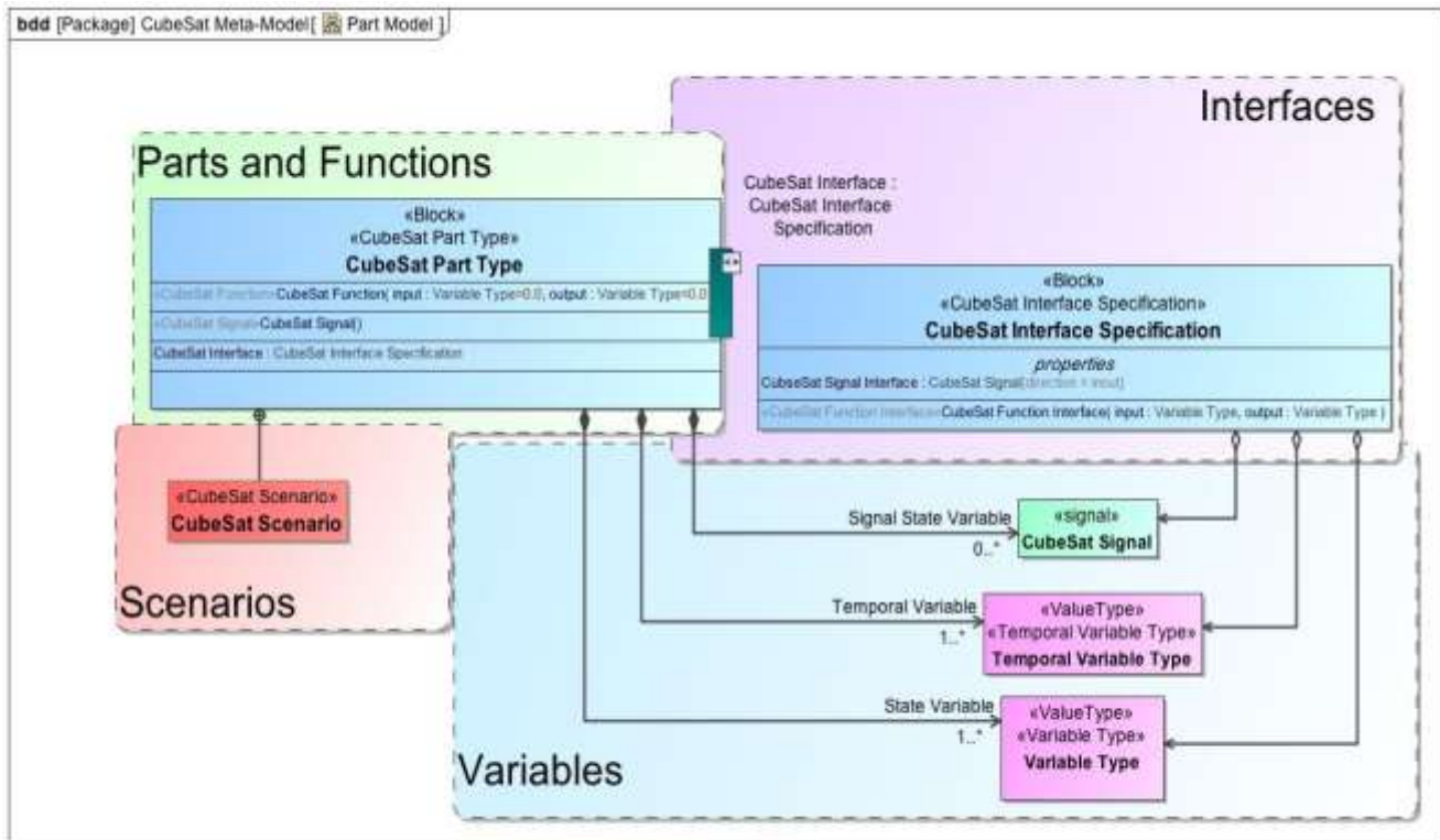
Figure 2. Pattern for Modeling CubeSat Framework
