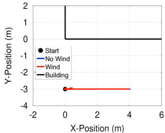
Figure 14. Ground track, 2 nd test profile, with relaxed small angle approximation
