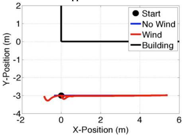
Figure 11. Ground track, 2 nd test profile
