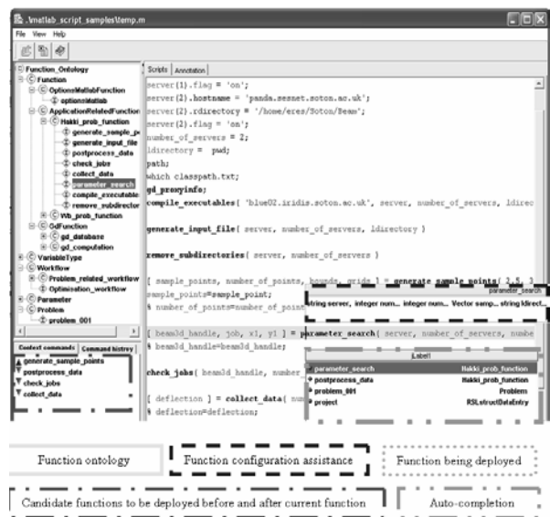
Figure 9 Domain script editor integrated with the advisor
