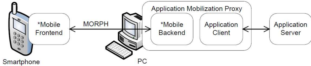
Figure 1: Network Architecture of *Mobile
