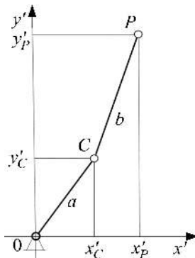
FIG. 2. Kinematic chain DCP.
