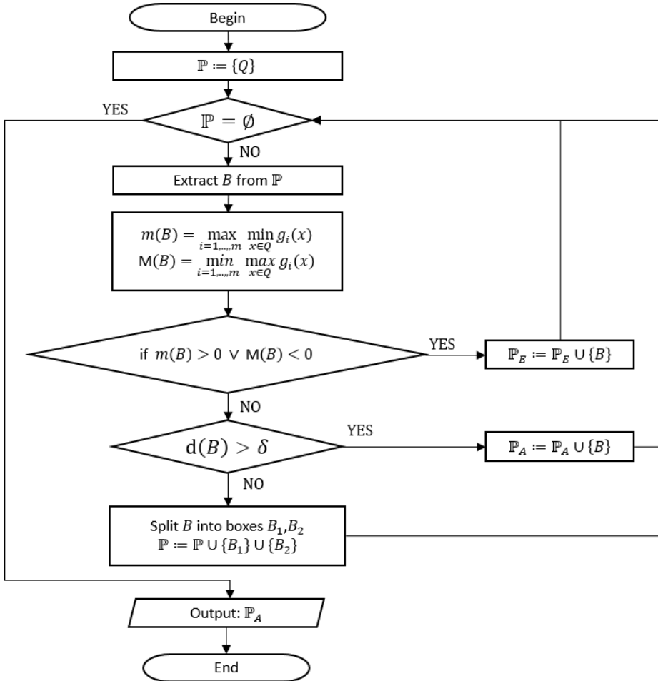
FIG. 3. Algorithm A for approximating a working area.
