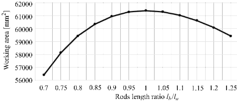
FIG. 6. The dependence of the area of the working area on the ratio of the length of the rods.
