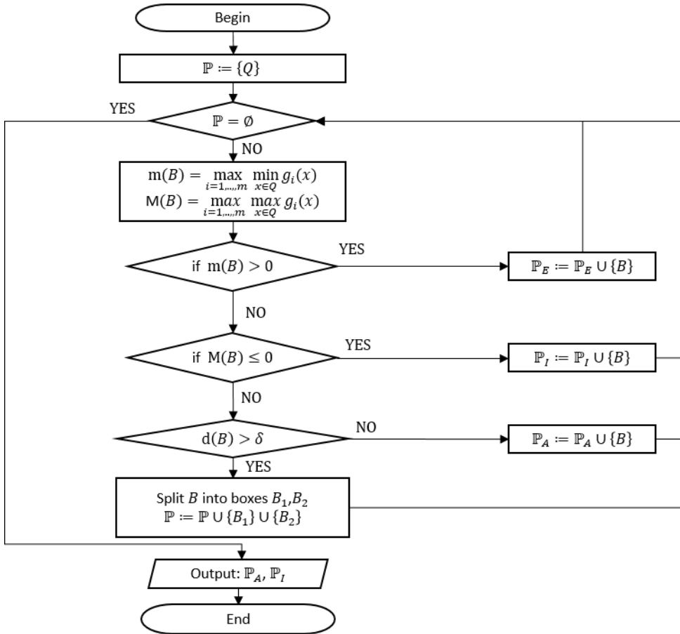
FIG. 4. The algorithm B for approximating the working area.
