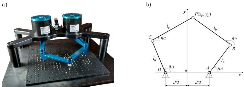
FIG. 1. Robot RRRRR : a) robot layout, b) block diagram of the robot.
