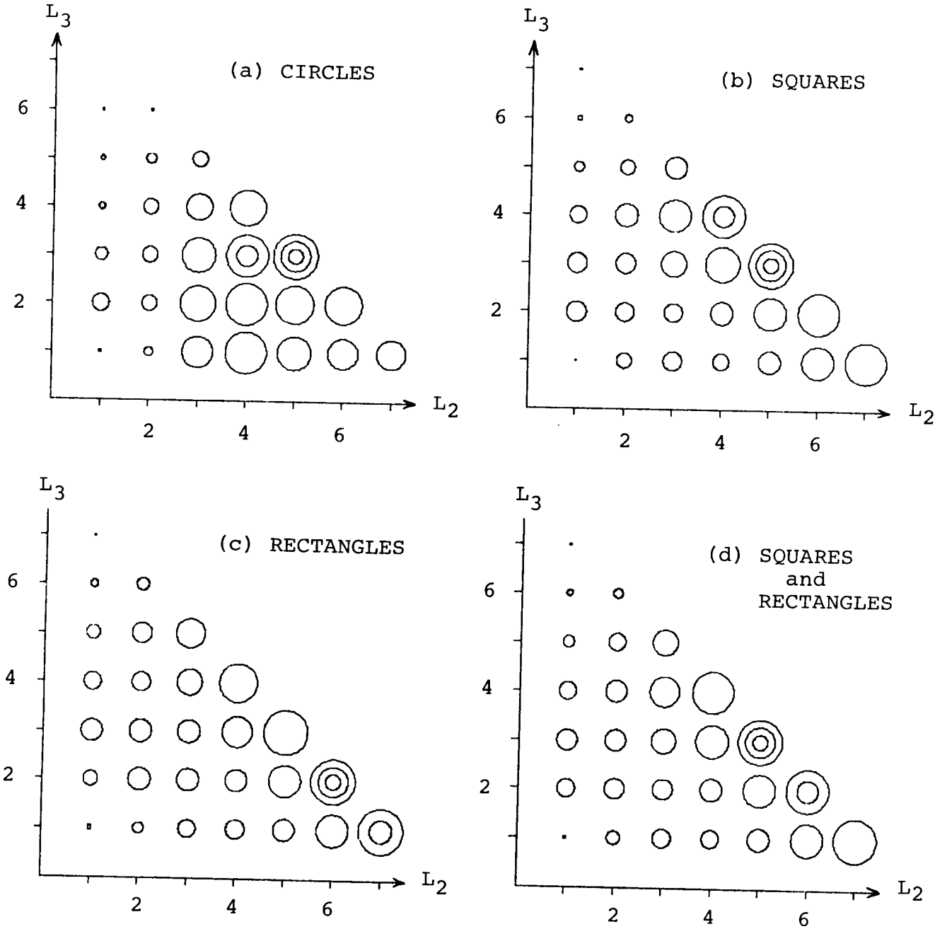
Figure 8: Simulated results of graspings under (W_r)_t > 0.8 , 0 < \theta_0 < \pi/2 and 0 < \theta_1 < \pi/2 .
