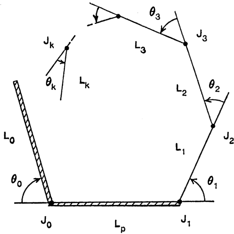
Figure 1: Finger structure.
