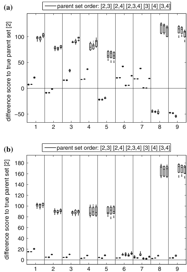
Fig. 7 Detailed Chib log marginal likelihood (MLL) scores for the original CheMA method with g-Prior (a) and a modified method with a ridge prior (b). Detailed plots from which the average score distributions in Fig. 6 are derived. Each of the nine slots along the horizontal axis corresponds to one parameter configuration of (v_{0,y}, k_{2,y}, v_{2,y}) as displayed in Table 3 and used for the synthetic data in Sect. 5.1. The slots contain the Chib MLL difference scores between a wrong parent configurations (the parent configurations are aligned from left to right in each slot according to the order in the legend) and the true parent set ([2]). Positive values indicate that the true parent configuration receives a higher score
