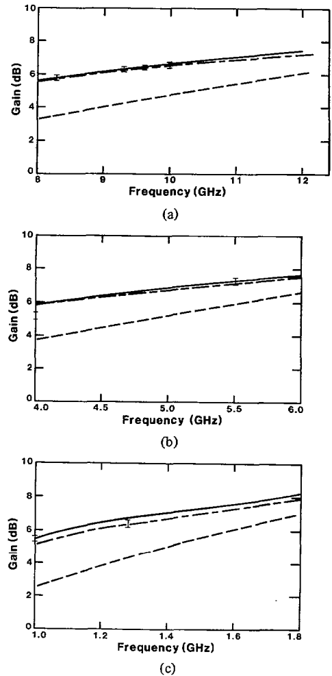
Fig. 7. On-axis gain of open-ended rectangular waveguide calculated from (13) (—), (15) (---), and the Stratton-Chu formulas (···). The I symbols denote NBS measured values of gain and estimated limits of error. (a) X-band, (b) C-band. (c) L-band.
