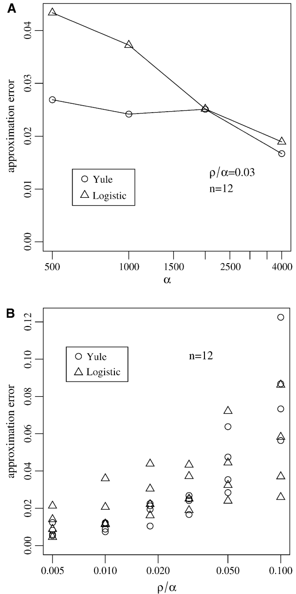
FIGURE 6.—Approximation errors \varepsilon_L^i and \varepsilon_Y^i for the sizes of the two biggest families that are identical by descent during the sweep for the Yule and the logistic models. Every point is based on 10^5 simulations of a sample of size 12 in the Wright-Fisher model with population size 10^5 and the corresponding approximating Yule and logistic models. (A) The ratio of recombination rate and selection strength \rho/\alpha = 0.03 is fixed and \alpha varies. (B) Several ratios \rho/\alpha were considered. For each of these ratios, \alpha = 500, 1000, 2000, and 4000 are considered. The values for \rho/\alpha = 0.03 are based on the simulations shown in A.
