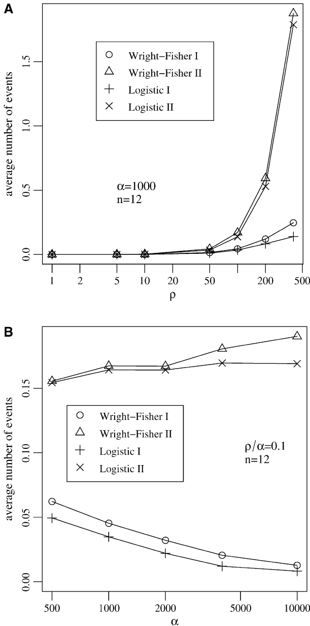
FIGURE 5.—Two kinds of events may occur backward in time in the genealogy of the linked neutral variant in the wild-type background: (I) coalescence events and (II) recombinations with a beneficial allele denoted by back-recombinations . (A) The average number of these events increases with the recombination rate \rho , but (B) for fixed \rho/\alpha stays bounded for a wide range of values of the selection strength \alpha . The Yule approximation does not allow for any of these events.
