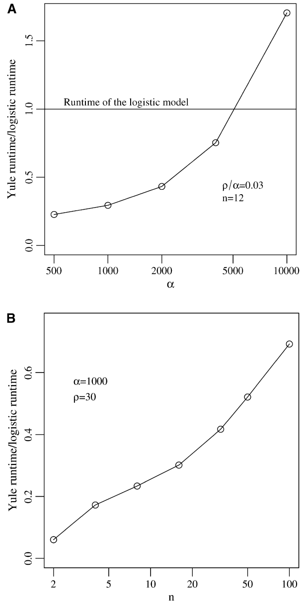
FIGURE 3.—Run-time ratios for simulating the logistic and Yule approximations. Run time depends on (A) the selection strength \alpha and (B) the sample size n .
