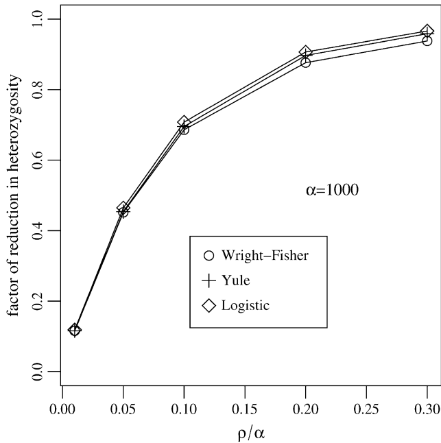
FIGURE 4.—Heterozygosity is reduced by a factor h depending on the selection strength, \alpha , and the recombination rate, \rho , during a selective sweep. Both theoretical predictions for the logistic and Yule model work well.
