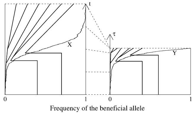
FIGURE 1.—(A) The coalescent for the neutral locus is generated conditioned on the frequency X of the beneficial allele. (B) The time change d\tau = (1 - X_t)dt transforms the process X to a supercritical branching process. The coalescent is also time changed. See text for explanation.
