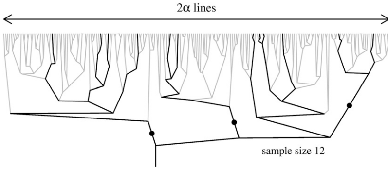
FIGURE 2.—A Yule tree approximating the genealogy of a selective sweep. The thick lines represent the genealogy of the sample; solid circles correspond to recombination events along the branches. See text for explanation.
