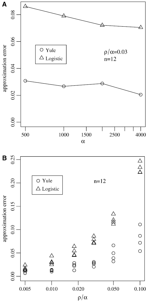
FIGURE 7.—Approximation errors \varepsilon_L and \varepsilon_Y for the number of lineages going back to the founder of the sweep and the size of the largest recombinant family for the Yule and the logistic models. The same simulations and parameter combinations as in Figure 6 were used.
