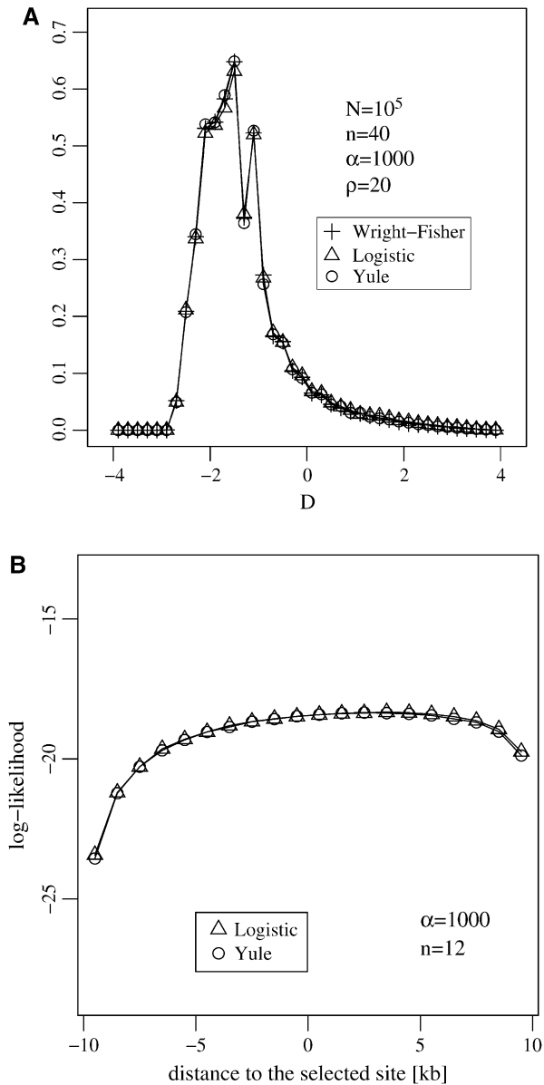
FIGURE 8.—(A) The distribution of Tajima's D estimated at the end of a selective sweep by simulating the Wright–Fisher model and the logistic and the Yule approximations during the selective phase. (B) The log-likelihood curve for the position of a selected locus given data from two adjacent neutral loci. The position of the selected site is at 0.
