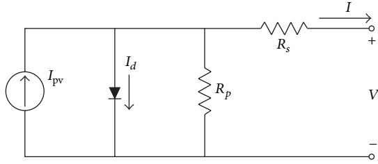
FIGURE 2: Circuit diagram of the SDM.
