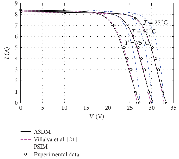
FIGURE 5: Current-voltage curves of a KC200GT PV module at various cell temperatures.
