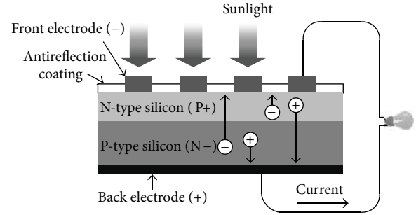
FIGURE 1: The basic structure of a silicon-based PV cell and its working mechanism.
