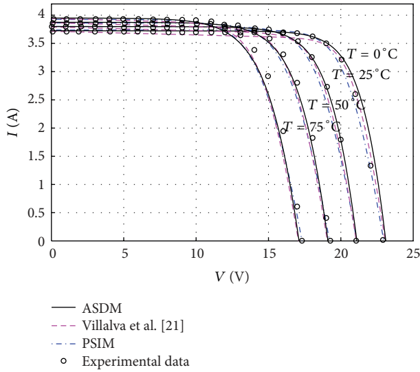
FIGURE 3: Current-voltage curves of a MSX60 PV module at various cell temperatures.
