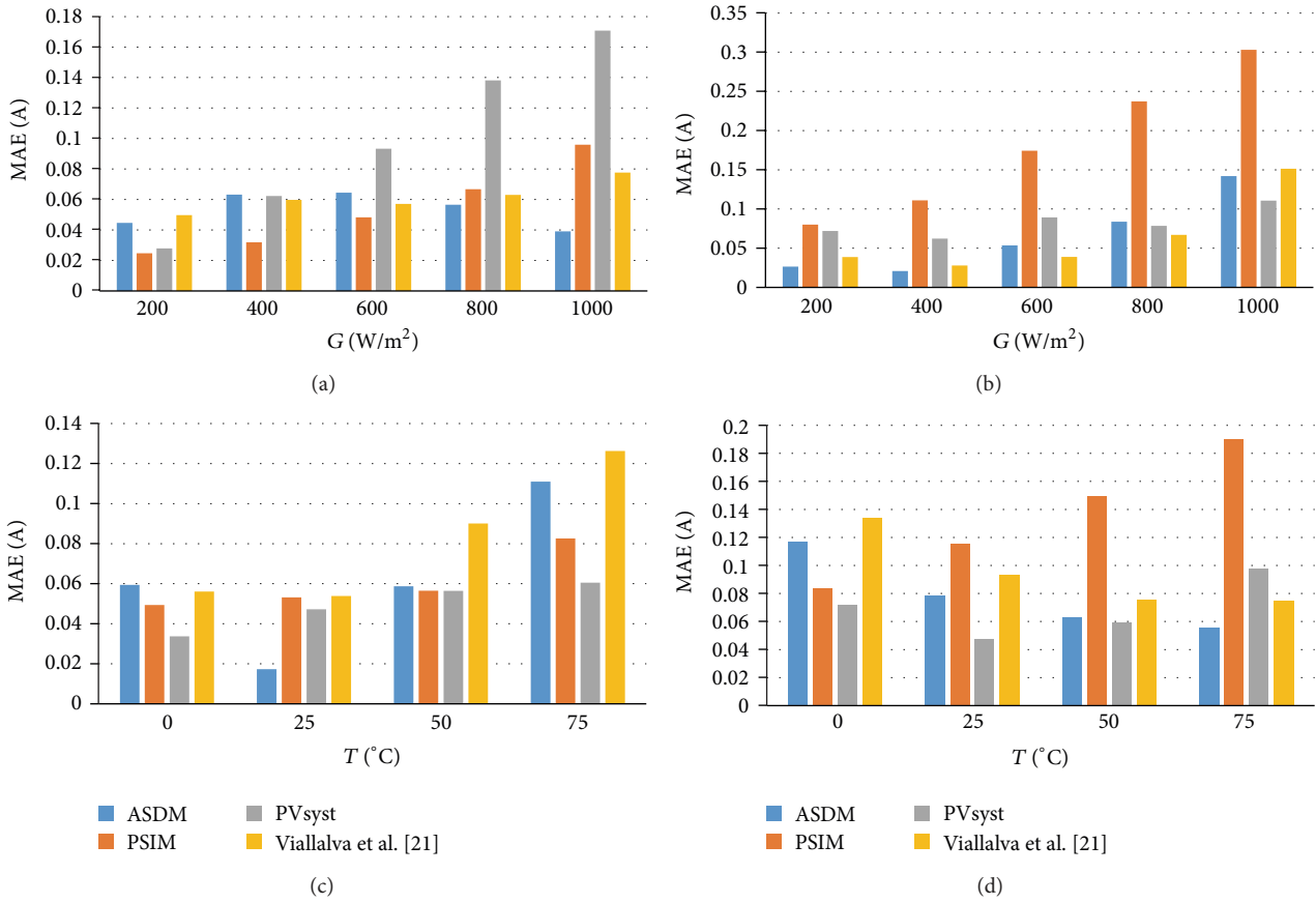
FIGURE 6: Mean absolute errors of the PV models at different atmospheric conditions: (a) SQ150-PC; (b) MSX60; (c) KC200GT; (d) HIT 180.
