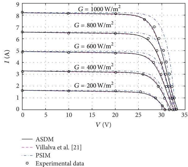
FIGURE 4: Current-voltage curves of a KC200GT PV module at various irradiance levels.
