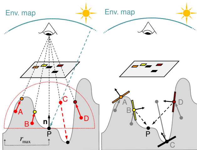
Figure 2: Left: For direct lighting with directional occlusion, each sample is tested as an occluder. In the example, point P is only illuminated from direction C. Right: For indirect light, a small patch is placed on the surface for each occluder and the direct light stored in the framebuffer is used as sender radiance.
