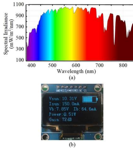
Fig. 10. (a) Solar spectrum measured during the field trial on the solar cell testbed located at KAUST ( 39^{\circ}06' E, 22^{\circ}17' N), and (b) photo of the display screen on the receiver circuit of AquaE-lite, where the output voltage ( V_{\text{sun}} ) and the current ( I_{\text{sun}} ) of the monocrystalline Si solar panel for energy harvesting were 10.31 V and 150.0 mA, respectively; the total consumed voltage ( V_b ) and current ( I_b ) of the two batteries on the receiver circuit of AquaE-lite were 7.85 V and 64.6 mA, respectively; the power consumed by the receiver circuit of AquaE-lite (Power) was 0.51 W; the PGA gain value (Gain) was 72 dB.
