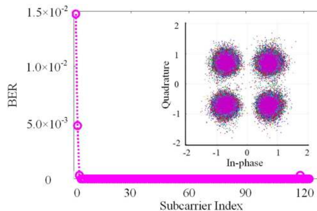
Fig. 11. BERs of the received 1.2-Mbit/s OFDM signals for different subcarriers after transmission through a 15-m air channel on the solar cell testbed located at KAUST ( 39^{\circ}06' E, 22^{\circ}17' N). Inset: the corresponding constellation map.
