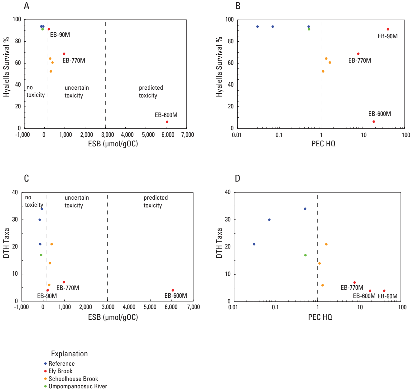
Figure 27. Comparison of sediment-quality criteria with various measures of sediment toxicity. A , The variation of Hyalella azteca survival in toxicity tests with the equilibrium-partitioning sediment benchmark (ESB). The boundaries between ESB ranges for no toxicity, uncertain toxicity, and predicted toxicity are from USEPA (2005). B , The variation of Hyalella azteca survival in toxicity tests with hazard quotients (HQ) based on the copper probable effects concentration (PEC). C , The variation of depositional-targeted habitat (DTH) taxa richness with the equilibrium-partitioning sediment benchmark (ESB). The boundaries between ESB ranges for no toxicity, uncertain toxicity, and predicted toxicity are from USEPA (2005). D , The variation of depositional-targeted habitat (DTH) taxa richness hazard quotients based on the copper probable effects concentration (PEC).
