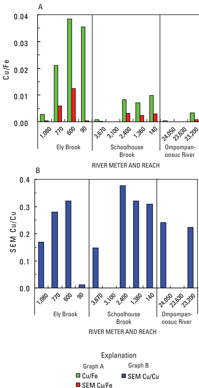
Figure 26. Copper (Cu) and iron (Fe) concentrations in stream sediments. Sites with no bars represent sites without samples. A , The variation within the watershed of the mass ratio of total Cu to total Fe, and the mass ratio of labile (SEM) Cu to total Fe. B , The variation within the watershed of the ratio labile (SEM) Cu to total Cu.
