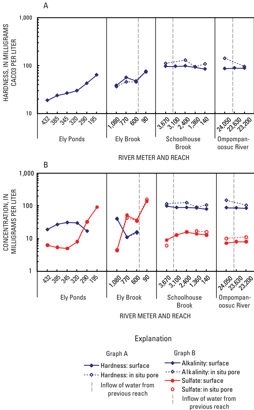
Figure 6. Downstream variations in (A) hardness, (B) alkalinity and sulfate concentrations in surface and in situ pore waters at the Ely Mine Superfund site, Vershire, VT.
