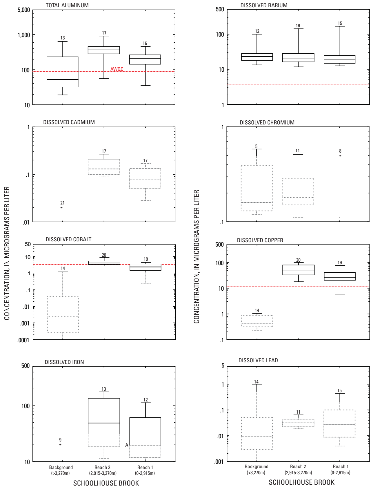
Figure 17. Select constituent concentrations in surface waters among three reaches in Schoolhouse Brook at the Ely Mine Superfund site, Vershire, VT. Data are from this study and Argue and others (2008).
