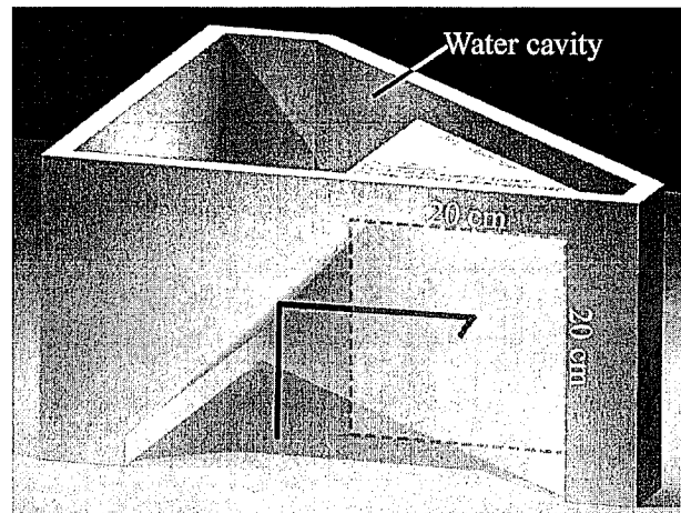
Fig. 2. (Color online) Trimetric rendering of the manufactured ABC source. The 20 cm \times 20 cm entrance aperture is highlighted by the dashed square and translucent overlay, and the geometric path is indicated by the heavy solid lines. The mirror is omitted for clarity.
