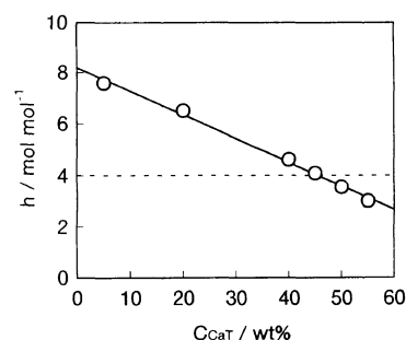
Figure 1. Calcium thiocyanate concentration C_{\text{CaT}} dependence of the number of solvated water molecules h in aqueous calcium thiocyanate solution at 60°C.
