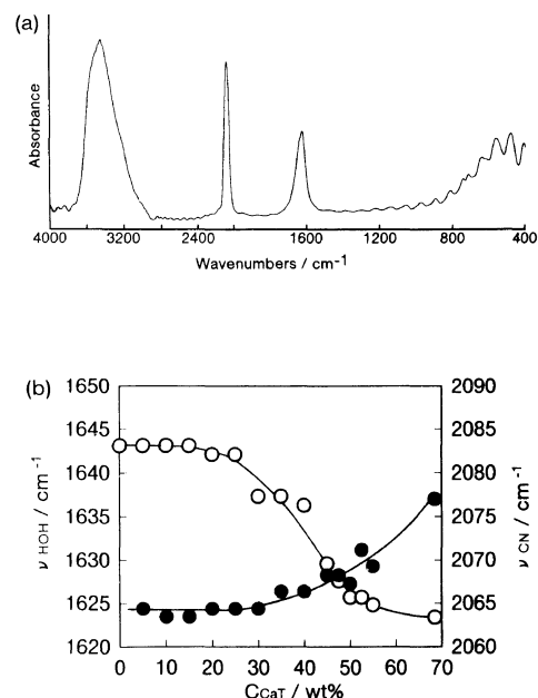
Figure 5. IR spectrum of aqueous calcium thiocyanate solution (a) and concentration C_{CaT} dependence of wave number of HOH bending ( \nu_{HOH} , \circ ) and CN stretching ( \nu_{CN} , \bullet ) vibration (b).
