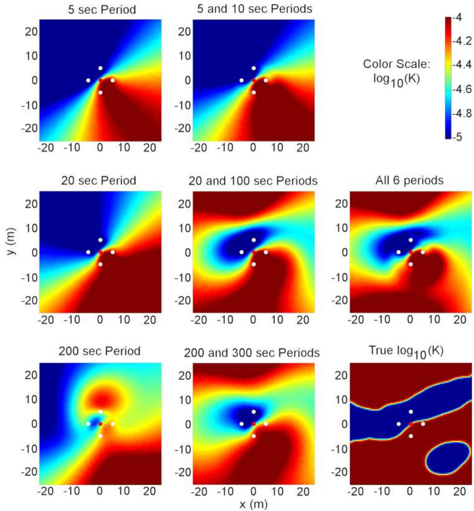
Figure 10. Comparison of inversion results obtained for representative single-frequency and multifrequency inversions. Area shown is the central 50 m × 50 m area of the synthetic model. First column shows single-frequency inversions. Second column shows two-frequency joint inversions. Third column shows six-frequency joint inversion (second panel), and true parameter field (third panel). Color scale is the same for all images.
