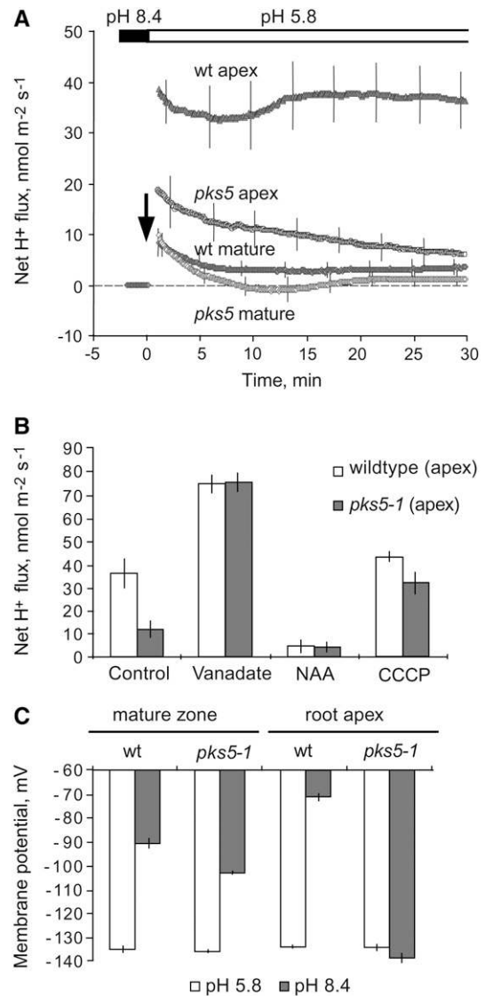
Figure 4. In Vivo Measurement of Net Proton Fluxes from Roots of pk5 and Wild-Type Plants.
