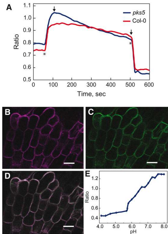
Figure 3. pH Ratio Imaging in the Apoplast of Columbia-0 and pk5-1 Roots.
