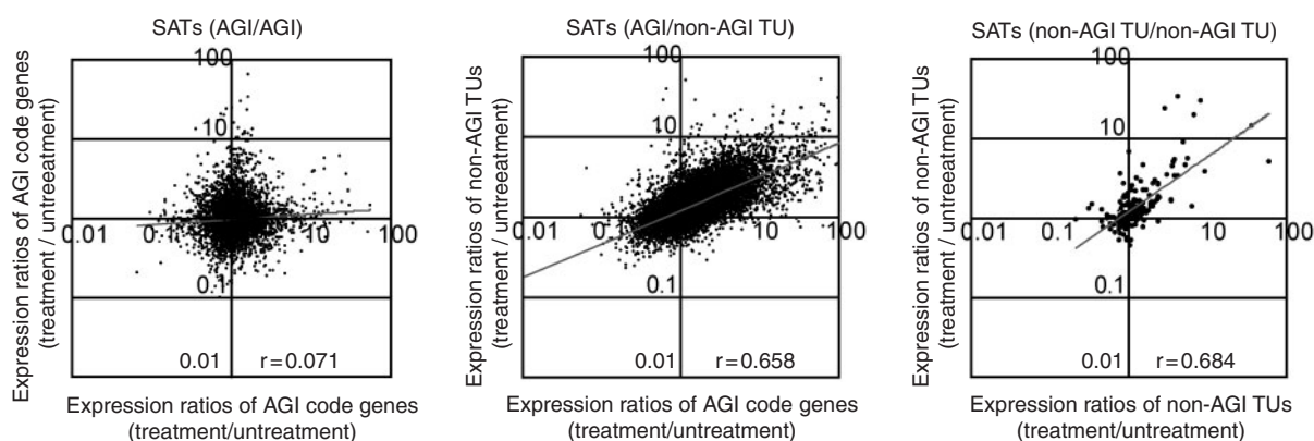
Fig. 2 The correlation of expression ratio (treated/untreated) between sense and antisense TUs of the SATs under drought, cold, high-salinity stress and ABA treatments. The log values for the expression ratios (stress and ABA treated/untreated) of sense and antisense TUs of the SATs were plotted. The left, middle and right panels represent the expression ratio in the SATs of AGI code/AGI code, AGI code/non-AGI TUs and non-AGI TUs/non-AGI TUs, respectively. In the left and middle panels, the X and Y axes represent the expression ratio of the AGI code genes (sense TUs) and the expression ratio of the TUs on the antisense strand, respectively. In the right panel, the X and Y axes represent the expression ratio of the non-AGI TUs (sense TUs) and the expression ratio of the TUs on the antisense strand, respectively. In each panel, the correlation coefficients are indicated.
