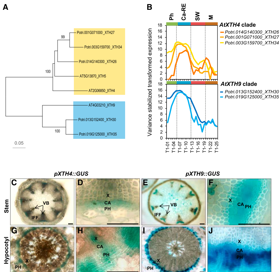
Figure 1. Clades AtXTH4 and AtXTH9 in Arabidopsis and Populus trichocarpa . A, Phylogenetic tree constructed using the neighbor-joining method of MEGA7 in default mode using MUSCLE-aligned protein sequences ( http://phylogeny.lirmm.fr/phylo.cgi/index.cgi ), with bootstrap test of 1,000 replicates shown in percentages beside branches. B, The expression patterns of P. trichocarpa members of AtXTH4 and AtXTH9 clades in different wood developmental zones ( http://aspwood.popgenie.org ). Ca-RE, Cambium-radial expansion zone; M, maturation zone; Ph, phloem; SW, secondary wall formation zone. C to J, AtXTH4 and AtXTH9 promoter activity in Arabidopsis mature inflorescence stems and hypocotyls as visualized by GUS histochemistry. In the inflorescence stems (C–F), the expression of both genes was detected in vascular bundles, whereas interfascicular fibers did not show any expression (C and E); the closeup vascular bundles (D and F) show signals in the vascular cambium, developing xylem, and developing and differentiated phloem. In hypocotyls (G–J), both genes were expressed in the region of secondary vascular tissue formation (G and I), encompassing the vascular cambium, developing secondary xylem and phloem, and recently differentiated phloem cells (H and J). CA, Vascular cambium; IFF, interfascicular fibers; PH, phloem; VB, vascular bundle; X, xylem. Bars = 50 \mu m.
