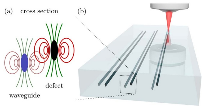
Figure 1 | Settings. (a) Idealised schematic showing the cross section of the waveguide arrangement where additional stress fields induce a reorientation of the waveguide's optical axis. (b) Sketch of the writing setting, with which the quantum gates are fabricated (here for 3 different orientations of the defect relatively to the waveguide). Higher pulse energies and lower writing velocity for the defects causes their missing light guiding properties and, hence, prevent loss due to coupling.
