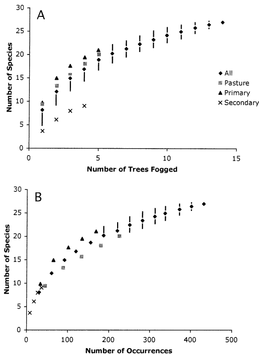
FIGURE 1. Species accumulation curves as a function of (a) number of trees fogged and (b) number of species occurrences in primary forest, secondary forest, relict pasture trees, and all three habitats combined. Curves are plotted from the means of 50 randomizations of sample accumulation order. Error bars on the combined curve are \pm 1 SD (omitted from parts of the curve to avoid clutter).
