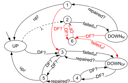
Figure 3. The failure model of a BC.
