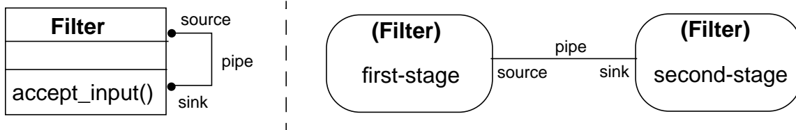
Figure 3: Naive object-oriented design (OMT) specification of simple pipe-and-filter system architecture.
