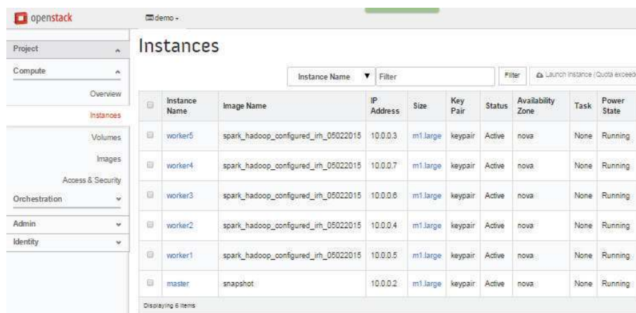
FIGURE 6: OpenStack GUI screenshot shows the cluster node specifications.
