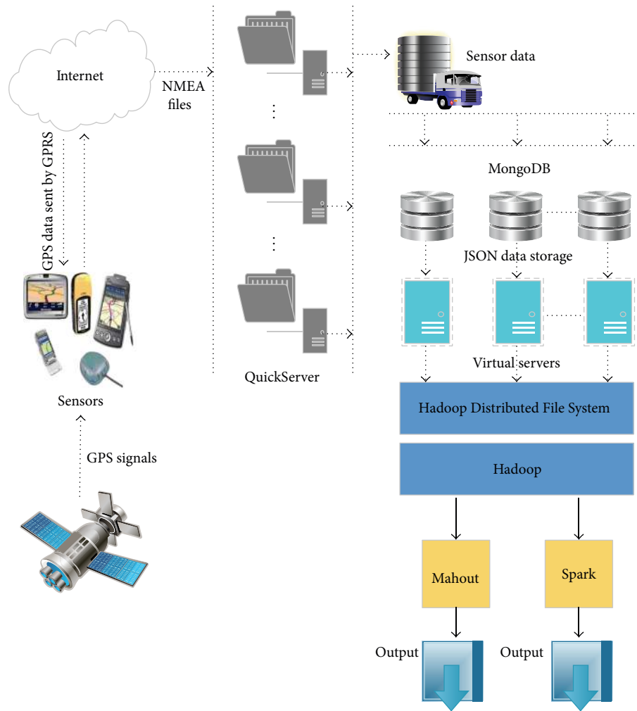
FIGURE 4: System architecture.
