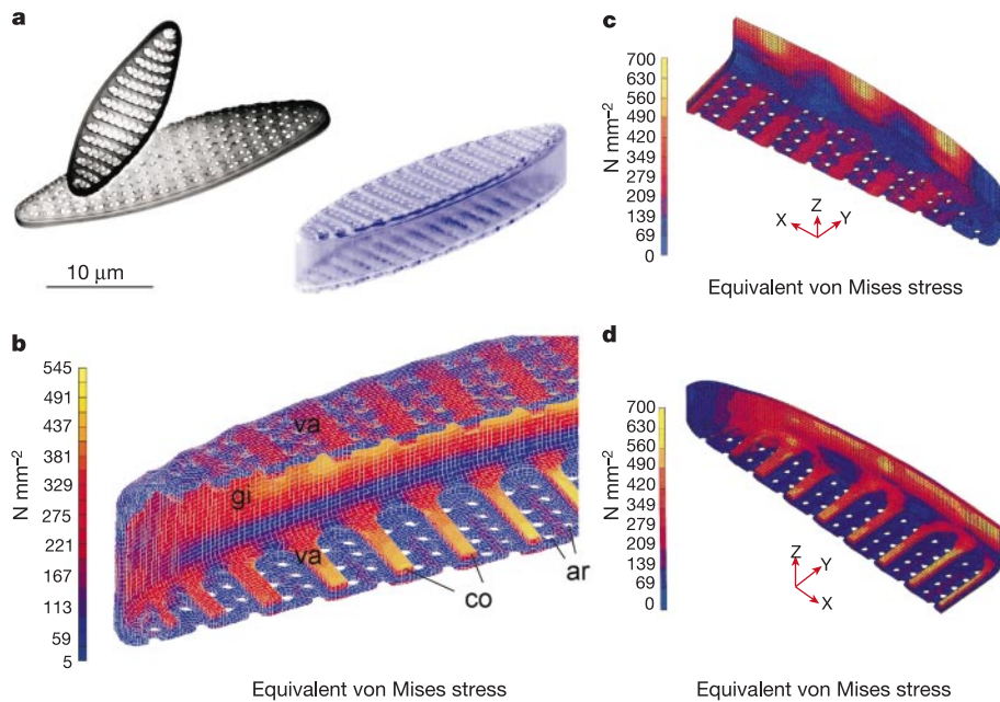
Figure 2 Finite element calculations of F. kerguelensis frustules. a , SEM of two valves (left) and rendered FEM of a complete frustule (right). b , Equivalent von Mises stress within the frustule as a function of pressure (total force, 750 \mu\text{N} ) on the girdle region. gi, girdle region; va, valve; co, costae; ar, areolae. c , d , One-eighth sections, external ( c ) and
