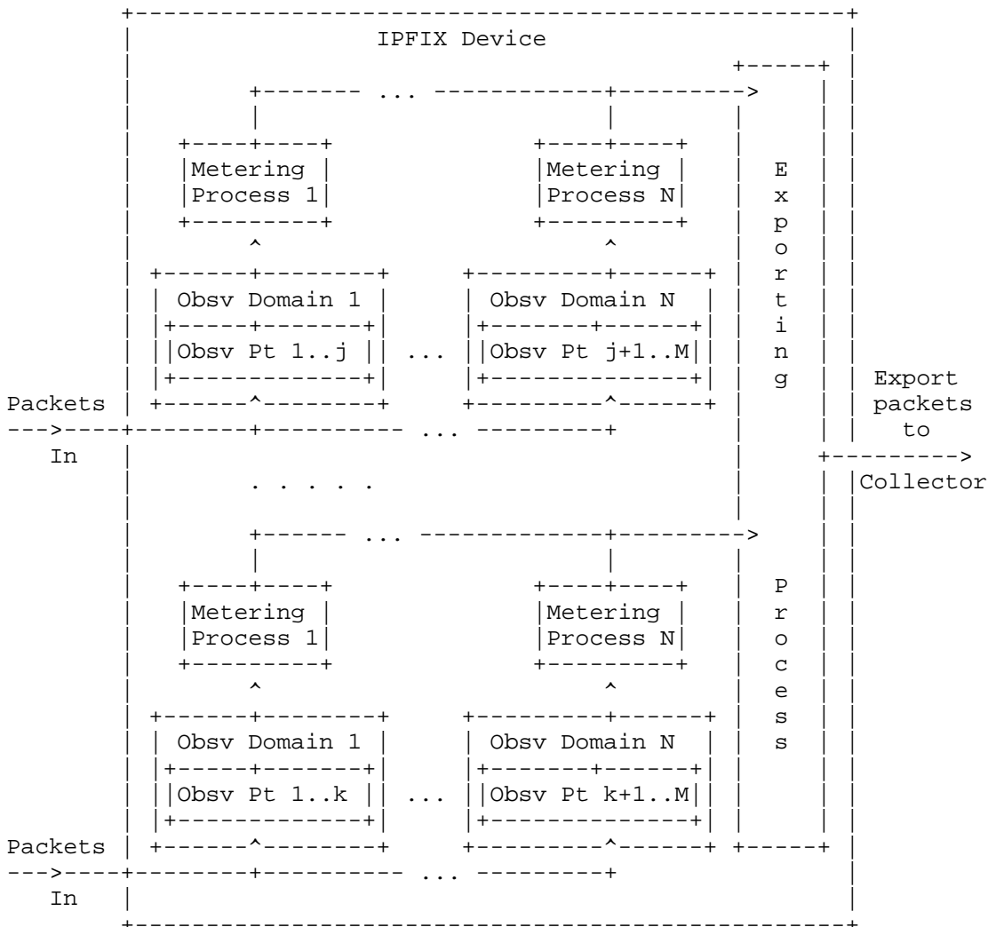
Figure 2: IPFIX Device
