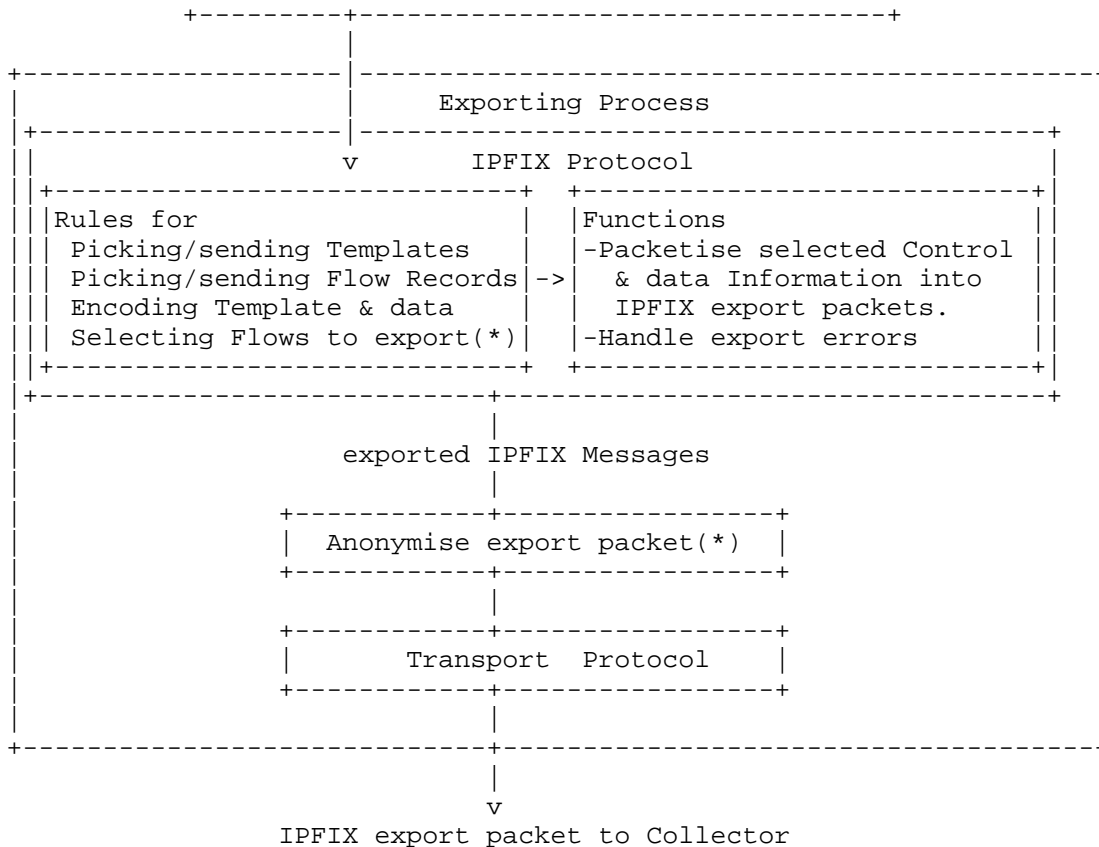
Figure 4: IPFIX Device functional blocks
