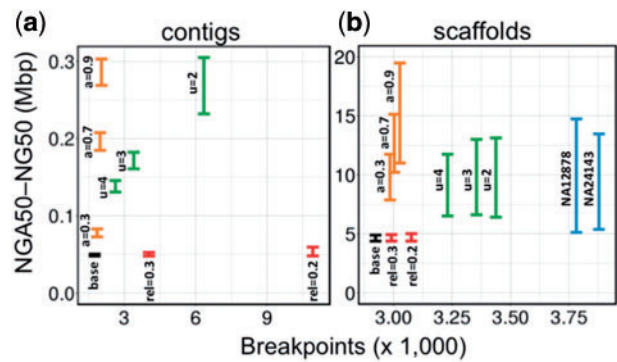
Fig. 2. Assembly contiguity and correctness from scaffolding (a) contig or (b) scaffold baseline assemblies with 10\times G Chromium reads using ARCS (orange), Architect (red) and fragScaff (green). We show the effect of the scaffolding parameters -a (ARCS), -rc-rel-edge-thr (abbreviated rel, Architect) and -u (fragScaff). The Y-axes show the range of NGA50 to NG50 lengths to indicate the uncertainty caused by real genomic variations (captured by breakpoints analysis) between individual NA24143 and the reference genome GRCh38. For comparison, we also show the same metrics for the Supernova assembly of the NA12878 and NA24143 10\times G datasets (blue). The X-axes show the number of breakpoints that occur when aligning the resulting assembly to the reference
