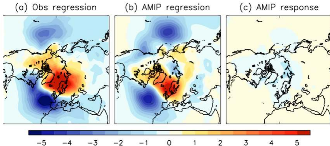
Figure 13. Linear regression between autumn (September–November) Arctic sea ice extent and winter (December–February) mean sea level pressure (reversed sign) in (a) observations and (b) atmosphere model experiments forced by observed sea ice and sea surface temperatures following the Atmosphere Model Intercomparison Project (AMIP) protocol. All time series were linearly detrended and cover the period December 1979 to November 2009. (c) Winter mean sea level response to reduced sea ice in atmospheric model experiments (scaled by the average autumn sea ice extent reduction). Units are hPa per million km 2 . (Figure from Smith et al. 2017).
