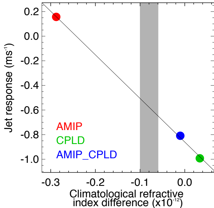
Figure 14. Dependence of Atlantic jet response on the background climatological refractive index difference between mid (25-35oN) and high (60-80oN) latitudes at 200 hPa. Grey shading shows the observed range from the ERA-Interim and NCEP II reanalyses. The Atlantic jet response is defined as the difference in zonal mean zonal wind at 200 hPa over the region 60-0oW, 50-60oN between model experiments with reduced and climatological Arctic sea ice. Experiments were performed with the same model but with three different configurations: atmosphere only (AMIP); fully coupled (CPLD); and atmosphere only but with SST biases from the coupled model (AMIP_CPLD). An “emergent constraint” is obtained where the observed refractive index difference (grey shading) intersects the simulated response (black line), suggesting a modest weakening of the Atlantic jet in response to reduced Arctic sea ice (Figure from Smith et al. 2017).
