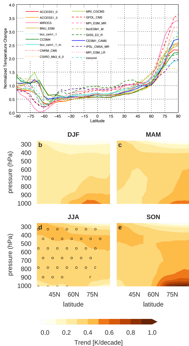
Figure 4. CMIP5 models simulations of (a) zonal-mean temperature changes normalized by the global mean change (2080-2100 minus 2005-2025) and (b-e) same as Figure 1b-e but for the CMIP5 multi-model mean historical + RCP8.5 for 1981-2015. Stippling indicates trends significant with a p < 0.05 after the false discovery rate was applied (Wilks 2006).
