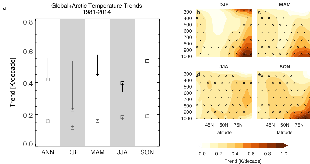
Figure 1. (a) Annual (ANN) and seasonal (DJF, MAM, JJA, SON) surface air temperature (SAT) trends from 1981 to 2014 in the Arctic (black squares, north of 60°N) and for the whole globe (gray squares) using the average of four observational products (CRU, NOAA, GISS, and BEST) masked in such a way that all four products share a uniform missing data mask over the ocean. The vertical lines show trends for the average of CRU and BEST without applying this uniform mask. This line therefore indicates, in large part, the uncertainty coming from the limited observational temperature record over the Arctic ocean. (b-e) Seasonal and zonal-mean air temperature trends from 1981-2015 for the average of the MERRA, MERRA-2, ERA-Interim, JRA-55, and CFSR reanalysis products. Stippling indicates trends significant with a p < 0.05 after the false discovery rate was applied (Wilks 2006).
