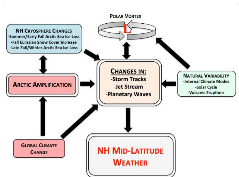
Figure 5. Complexity of linkage pathways. (Figure from Cohen et al. 2014).
