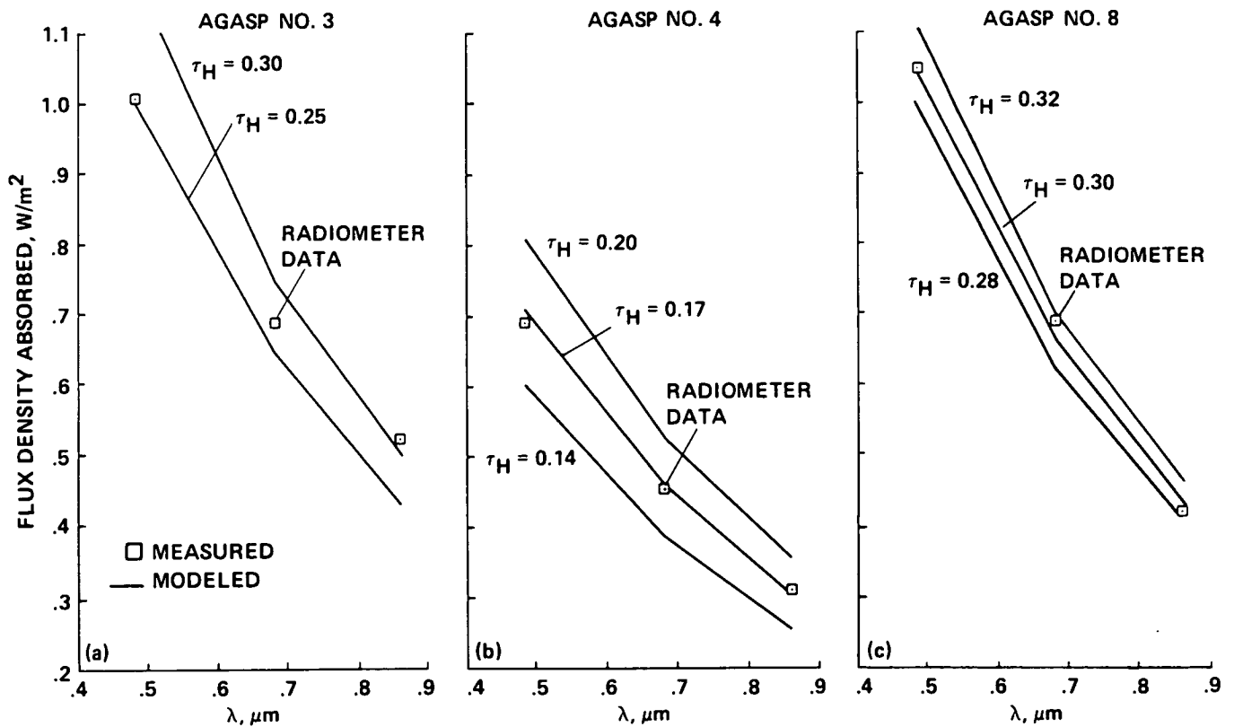
Figure 6.- Measured and calculated total power absorbed by the atmosphere in 0.01 \mu\text{m} intervals. \tau_H is the extinction optical depth at 500 nm. Symbols are measured values, solid lines represent model results.
