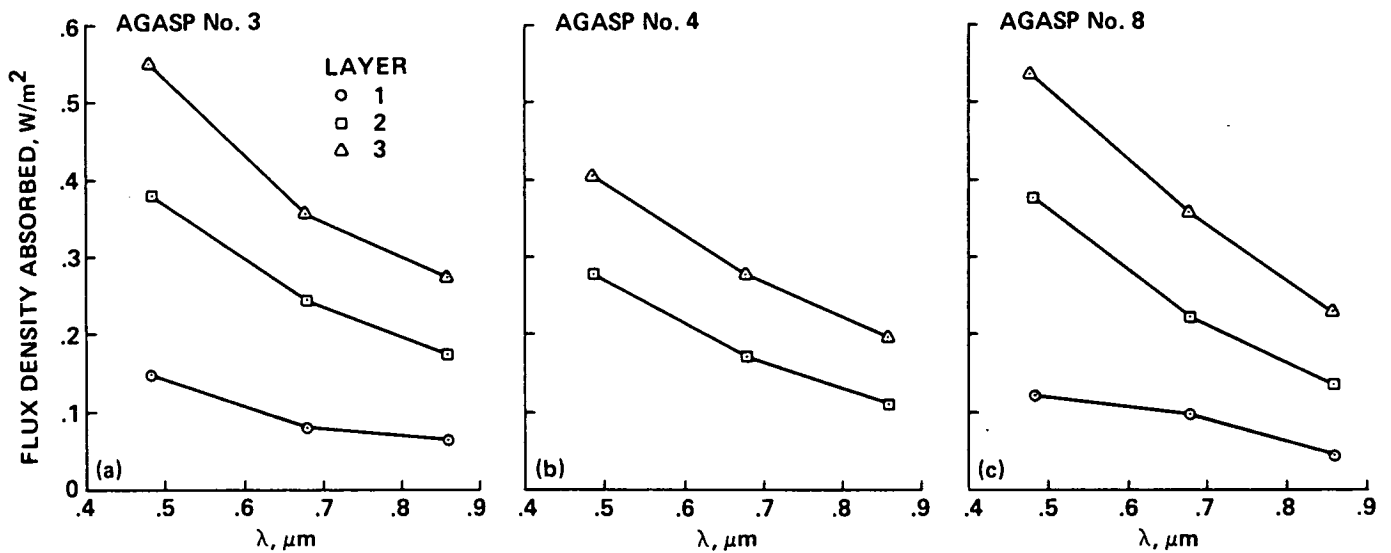
Figure 5.- Radiative power absorbed in 0.01 \mu\text{m} spectral bandpasses as a function of wavelength. Layers are defined in Table 1.
