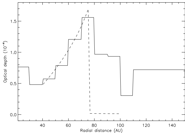
Figure 9. Optical depth in the \beta Pictoris debris disc derived from mid-IR imaging (Telesco et al. 2005). Overplotted is the \tau_{\text{eff}} profile for a secular-stirred planetesimal belt (dashed line) between 40–100 au (see text for details).
