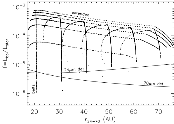
Figure 3. Evolution of narrow belts and extended discs (as labelled) in f versus r_{24-70} space from 1 Myr to 1 Gyr. Disc r_{24-70} increases as stirring moves outwards (so evolution is left to right). Here, f is derived from a blackbody at r_{24-70} (i.e. what detection at 24 and 70 \mu\text{m} would imply). Solid lines show 24 and 70 \mu\text{m} blackbody detection limits from Wyatt et al. (2007b). Extended discs have r_{\text{in-out}} = 15\text{--}120 au and \eta = 0.05\text{--}1.05 . For belts r_{\text{mid}} = 20, 30, 40, 50, 60 and 70 au, dr = r_{\text{mid}}/2 and \eta = 1 . Belts increase in radius from left to right, and extended discs increase in f with higher \eta . Other model parameters are as in the left-hand panel of Fig. 2.
