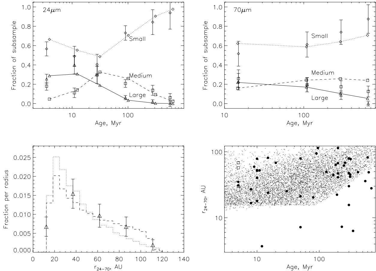
Figure 8. The best fit of the model population to 24 and 70 \mu\text{m} statistics with narrow belts. Top left- and right-hand panels: binned 24 and 70 \mu\text{m} evolution; lower left-hand panel: overall (dashed line) and detectable (dotted line) model r_{24-70} (omitting the four possibly transient sources noted in the text), and lower right-hand panel: r_{24-70} versus t compared to the 46 star subsample (open squares show three additional sources detected by Carpenter et al. 2009, HIP 76310, HIP 77911 and HIP 80088).
