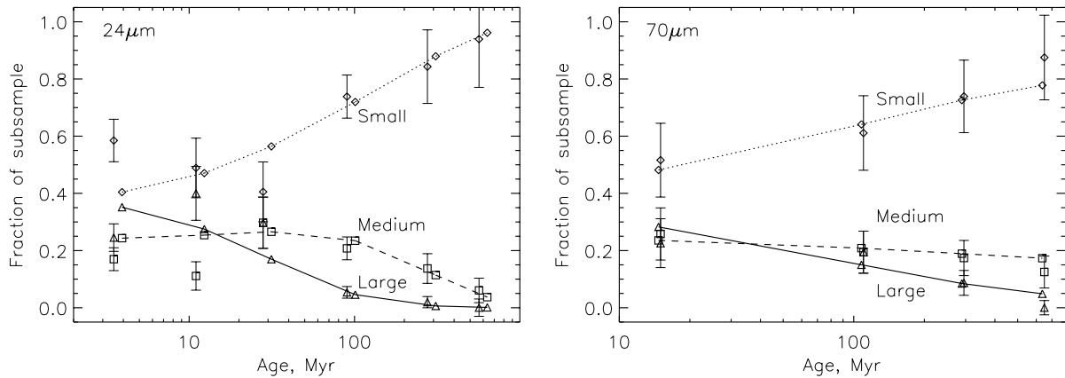
Figure 6. Best-fitting parameters for the Wyatt et al. (2007b) pre-stirred model at 24 and 70 \mu\text{m} (same symbols as Fig. 4, joined by solid, dashed and dotted lines for large, medium and small excesses, respectively). Symbols with error bars show observed A-star statistics. At 24 \mu\text{m} , the model predicts too many stars with large excesses at the earliest times, and a monotonic decline in the overall fraction of stars with excesses. There are no new 70 \mu\text{m} data so the right-hand panel is the same as Wyatt et al. (2007b) Fig. 2.
