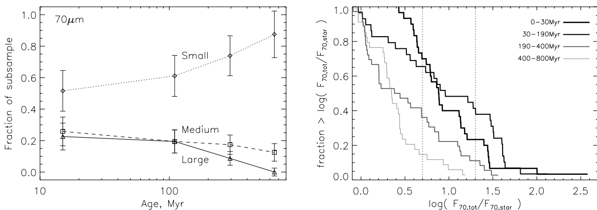
Figure 5. Same as in Fig. 4, but for 70\ \mu\text{m} excesses.
