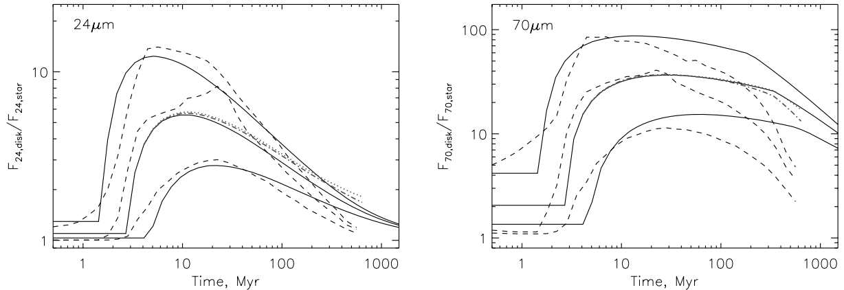
Figure 1. Evolution of 24 \mu\text{m} (left-hand panel) and 70 \mu\text{m} (right-hand panel) excesses for \eta = 1/3, 1, and 3 for a disc from 30 to 150 au from our model (solid lines) compared to models from Kenyon & Bromley (2008) (dashed lines), for an A2 ( 2.5 M_{\odot} ) star. The main difference between the models at 70 \mu\text{m} is caused by continued accretion and subsequent stirring in the Kenyon & Bromley (2008) models (see text). Also shown is the effect of the increasing main-sequence luminosity on an \eta = 1 disc with D_{\text{bl}} = 1 \mu\text{m} (grey dotted line) and then also allowing D_{\text{bl}} to vary (grey dot-dashed line). The overall effect of stellar evolution due to changing D_{\text{bl}} and hotter grains (i.e. dot-dashed line) is a small increase in 24 \mu\text{m} excesses and a similar decrease in 70 \mu\text{m} excesses.
