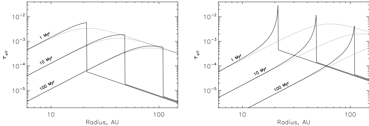
Figure 2. Evolution of \tau_{\text{eff}} for self-stirred (solid lines) and pre-stirred (dotted lines) discs at 1, 10 and 100 Myr. In the left-hand panel t_c \gg t_{\text{stir}} , so evolution is ‘slow’ and similar to the pre-stirred case. In the right-hand panel t_c \ll t_{\text{stir}} so the evolution at r_{\text{stir}} is ‘fast’ and much more violent as the disc reverts to the equilibrium state. Lines are offset slightly to remove ambiguities. The discs extend from 5–150 au around an A2 star and have parameters: \eta = 1 , Q_D^* = 150 \text{ J kg}^{-1} , e = 0.05 , x_{\text{delay}} = 0.01 and D_c = 60 \text{ km} (left-hand panel) and D_c = 1 \text{ km} (right-hand panel). The peak surface density is larger for the fast self-stirred disc because more mass is concentrated in smaller size objects.
