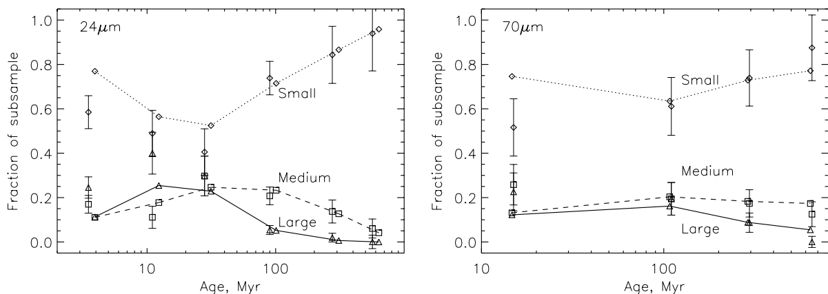
Figure 7. Simple delayed stirring model compared with 24 and 70 \mu\text{m} statistics. Symbols and lines are as in Fig. 6. All discs begin their evolution after \sim 10 Myr.
