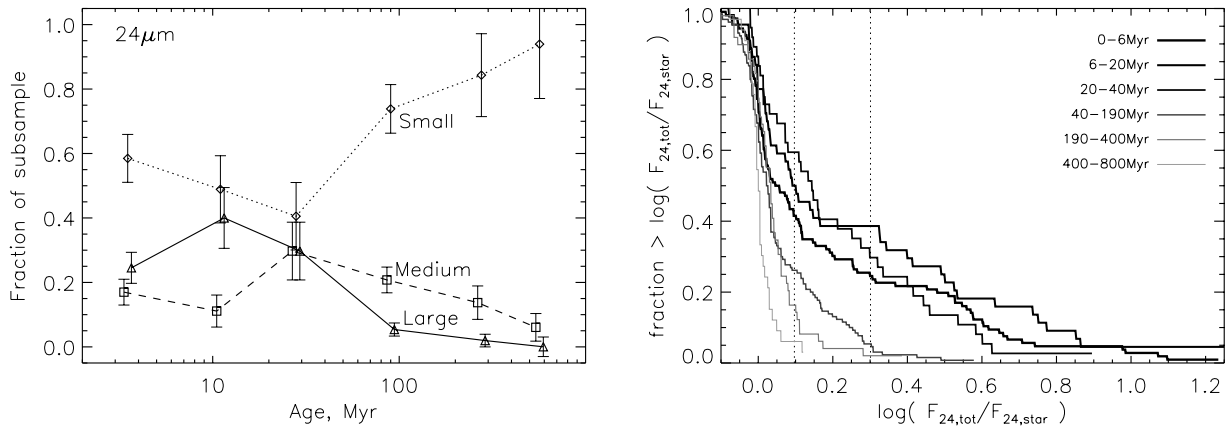
Figure 4. Evolution of A-star 24 \mu\text{m} excesses. The left-hand panel shows stars binned by age and large (triangles), medium (squares) and small (diamonds) excesses (ages offset slightly for clarity). Error bars are \sqrt{N} in each bin and for the oldest large excess bin we assume one disc to calculate the error. Excesses reach an overall peak around 30 Myr. The right-hand panel shows cumulative distributions of 24 \mu\text{m} excesses for the same age bins, from dark to light grey lines. The dotted lines indicate the bin edges for small, medium and large excesses. In the second youngest bin HR4796A and \beta Pic are beyond the right edge of the plot.
