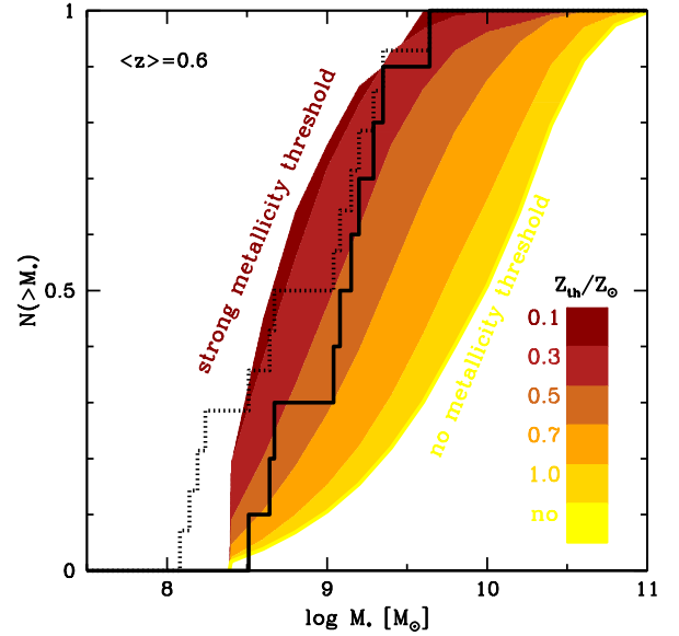
Fig. 5. Cumulative distribution of the stellar masses (including the old stellar population) of the LGRB hosts in our sample (dotted line: whole sample; solid line: with \text{Log } M_{\star} > 8.4 M_{\odot} , to comply with the simulation limits) compared to what is obtained by LGRB host galaxy simulations. The observed distribution is explained by a metallicity cut favouring low metallicities ( Z < 0.5 Z_{\odot} ).
