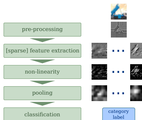
Figure 1: Architectural model of the classification pipeline. On the right side, the evolution of the internal representation is depicted for a sample truck image taken from the CIFAR-10 dataset [14].
