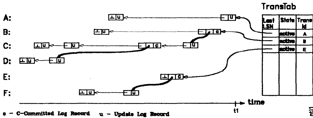
Figure 2: Log and TransTab at a Particular NBK-Subsystem
