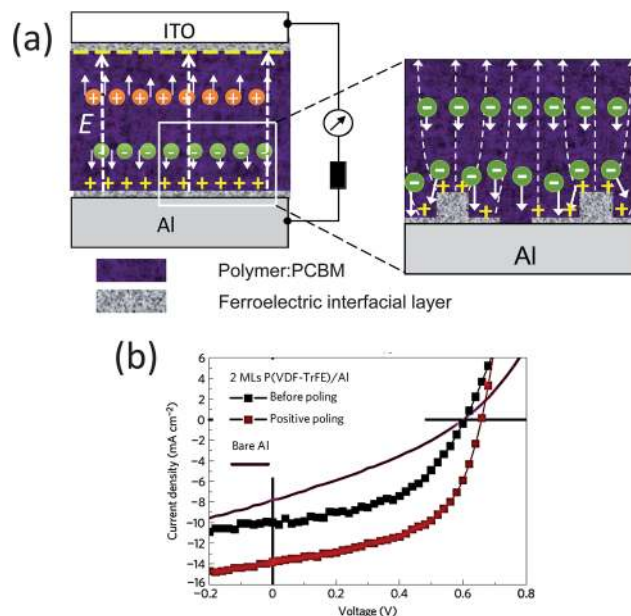
Fig. 6 (a) Schematics of FE-OPV and working principle with the ferroelectric polymer at the interface; (b) photocurrent curves of a poly(4,4'-dioctylthieno(3,2- b :2',3'- d )silole)-2,6-diyl- alt -(2,1,3-benzothiadiazole)-4,7-diyl (PSBTBT):phenyl-C71-butyric-acid-methyl ester (PC70BM) device without an FE layer (magenta line), with an FE layer before poling (black square line) and after poling (red squares). 40
