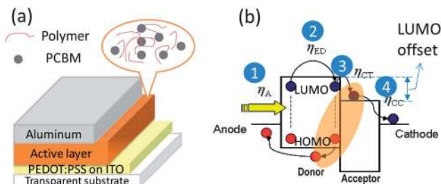
Fig. 5 (a) The device structure of a typical BHJ-OPV; (b) process of the conversion of incident light into electricity in OPVs. The electrons on the acceptor are still bound to holes on the donor right after the charge transfer, as illustrated by the ellipse in the figure.
