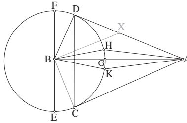
Fig. 4. Diagram for Prop. 4 (Heath 1913, 364). There is no X or BX in any MS. The line \widehat{BC} appears in the Arabic MSS but not in the Greek
