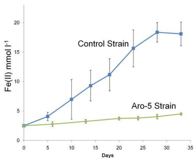
FIG 4 Fe(II) produced from Fe(III) oxide reduction over time in the Aro-5 and control strains. Results are the means and standard deviations of results from triplicate cultures for each strain.
