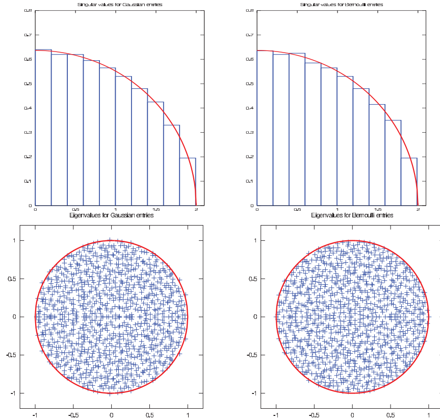
FIG 2. Illustration of universality in the quarter circular law and the circular law theorems 2.1 and 2.2. The plots are made with the singular values (upper plots) and eigenvalues (lower plots) for a single random matrix X of dimension n = 1000 . On the left hand side, X_{11} follows a standard Gaussian law on \mathbb{R} , while on the right hand side X_{11} follows a symmetric Bernoulli law on \{-1, 1\} . Since X has real entries, the spectrum is symmetric with respect to the real axis. A striking fact behind such simulations for the eigenvalues (lower plots) is the remarkable stability of the numerical algorithms for the eigenvalues despite the sensitivity of the spectrum of non-normal matrices. Is it the Śniady regularization of Brown measure theorem [137] at work due to floating point approximate numerics?
