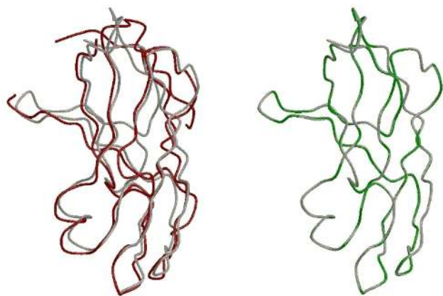
Figure 3 Left: a superposition of the search model (in red) for the eIAV dUTPase (§3.1) with the final structure (light grey). Right: the warpNtrace model in green superposed on the final structure (light grey).
