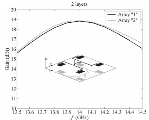
Fig. 16. Gain of the two interlaced arrays forming the dual polarized antenna.
