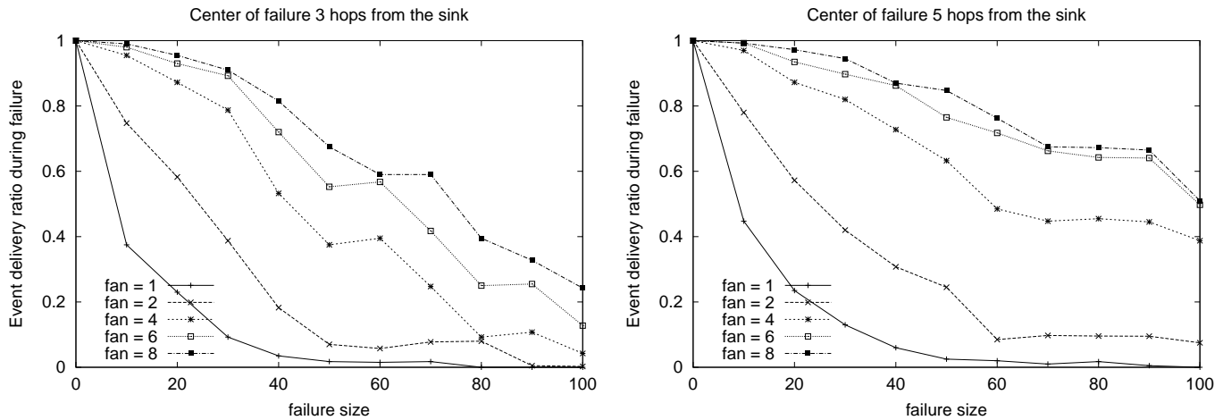
Fig. 7. Resilience to node failures: Effect of fanout size on event delivery ratio for various size failures. Failures were tested at two levels of the network: 3 and 5 hops from the sink.
