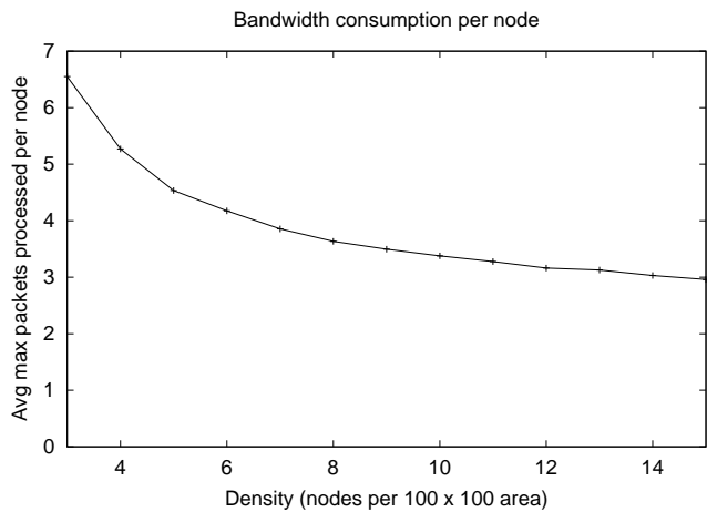
Fig. 4. Bandwidth: For eight sourced packets per event, this figure depicts the bandwidth consumption. One event occurs per simulation and the maximum number of packets processed by any given node for the entire simulation is recorded. The results of a series of simulations are averaged.
