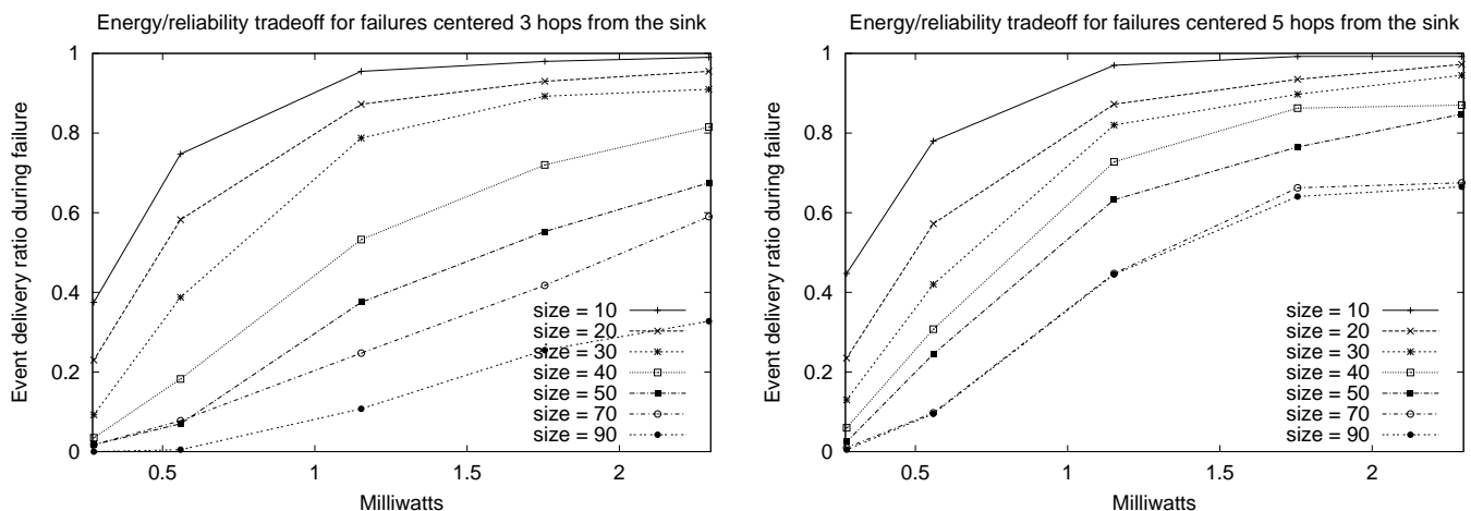
Fig. 8. Exploring the energy consumption/reliability tradeoff for various size failures. Energy consumption is the average energy consumption of the network per second during normal (failure free) operation. Reliability is the event delivery ratio during the failure period.
